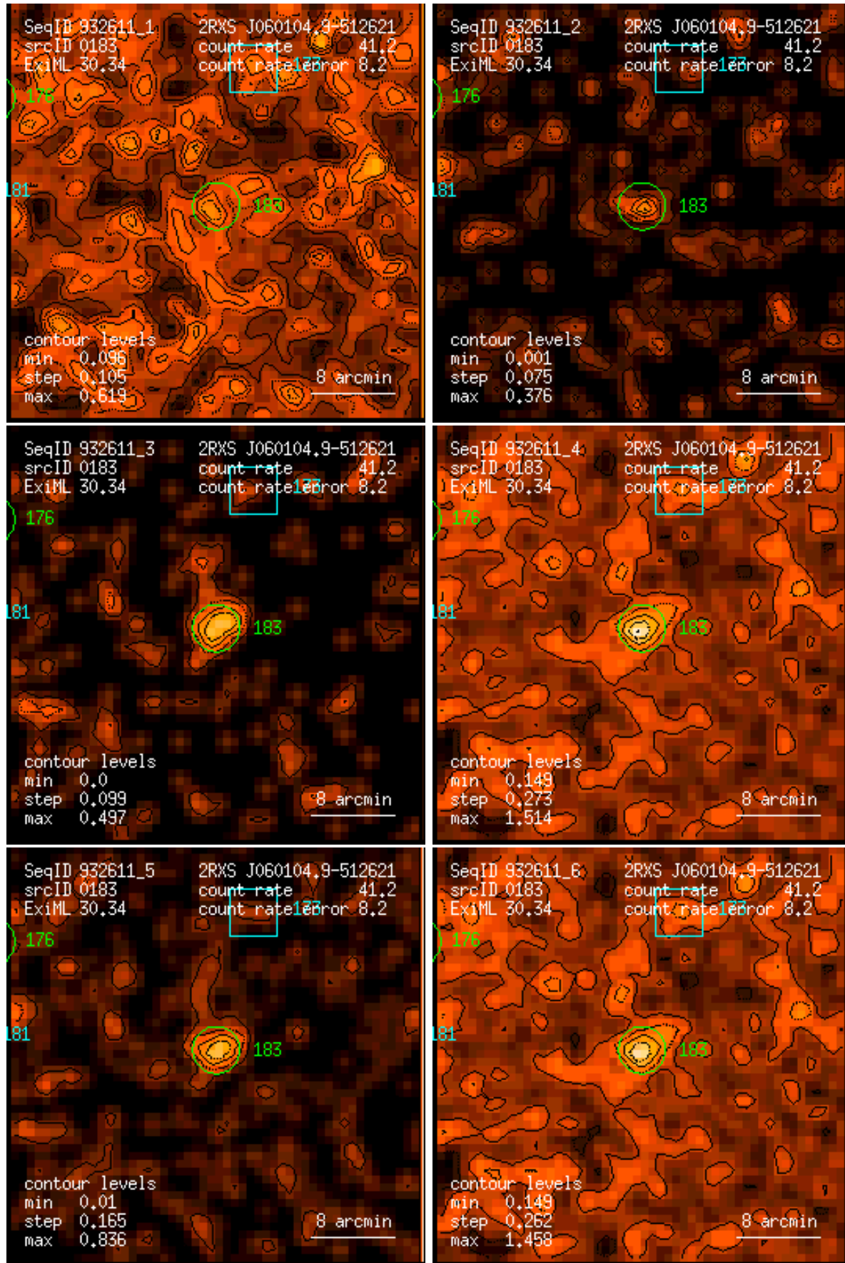
Figure 183: RASS 932611: detection 0183: band rate images, Gaussian filter: (1) PSPC channels 11 – 41, (2) 52 – 90, (3) 91 – 201, (4) 11 – 235, (5) 52 – 201, (6) 11 – 201. Broad band rates in counts/ks. Band rate contour levels in counts/ks/arcmin 2 .
