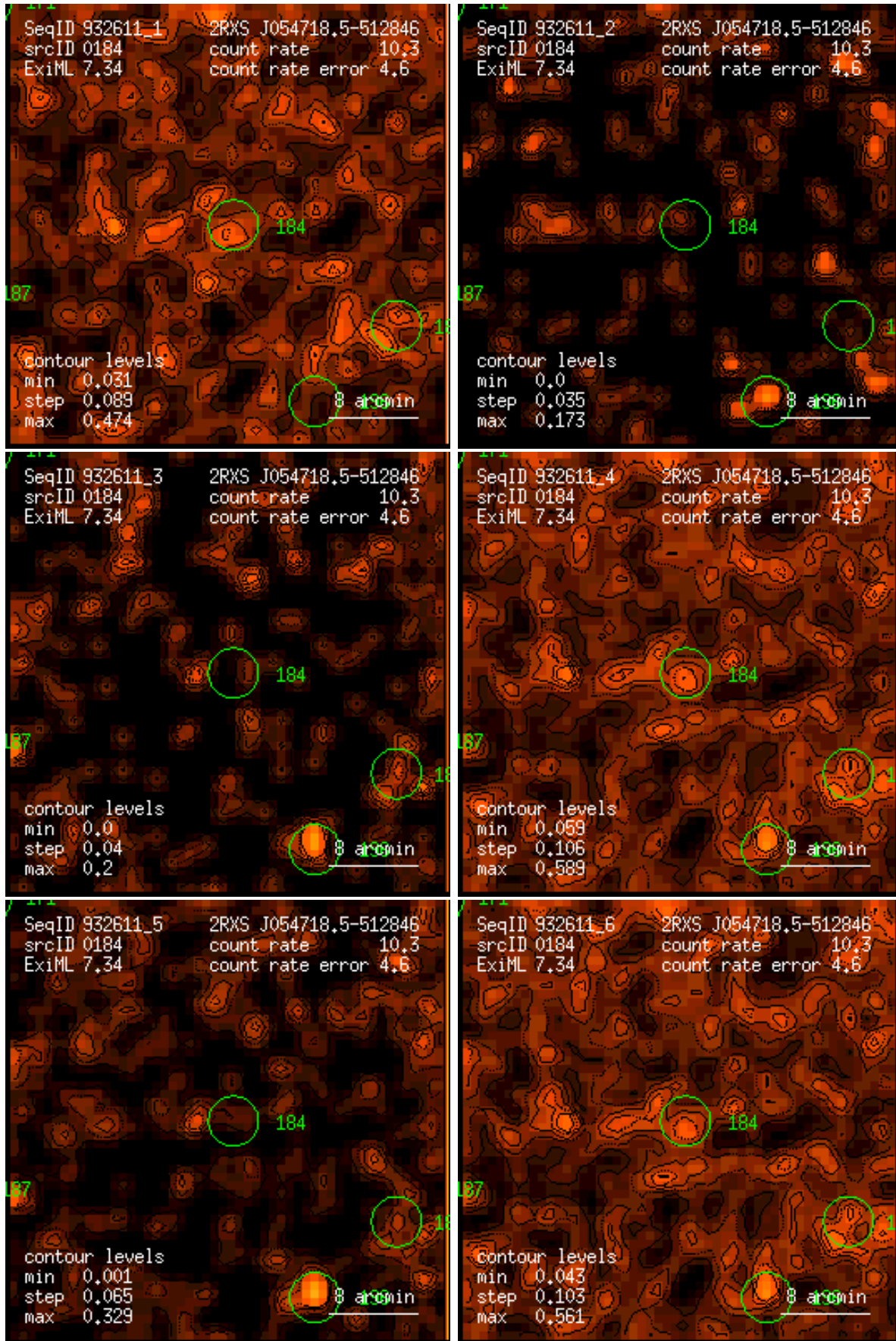
Figure 184: RASS 932611: detection 0184: band rate images, Gaussian filter: (1) PSPC channels 11 – 41, (2) 52 – 90, (3) 91 – 201, (4) 11 – 235, (5) 52 – 201, (6) 11 – 201. Broad band rates in counts/ks. Band rate contour levels in counts/ks/arcmin 2 .
