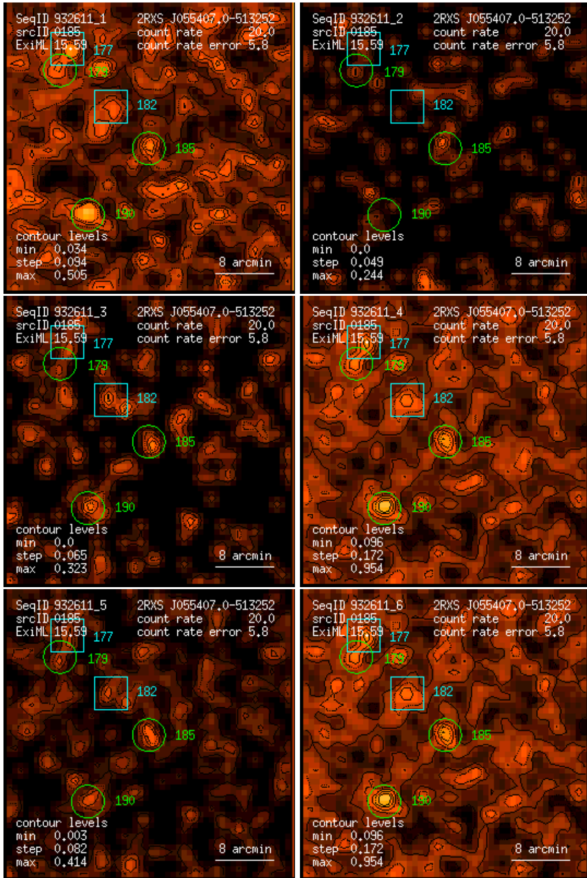
Figure 185: RASS 932611: detection 0185: band rate images, Gaussian filter: (1) PSPC channels 11 – 41, (2) 52 – 90, (3) 91 – 201, (4) 11 – 235, (5) 52 – 201, (6) 11 – 201. Broad band rates in counts/ks. Band rate contour levels in counts/ks/arcmin 2 .
