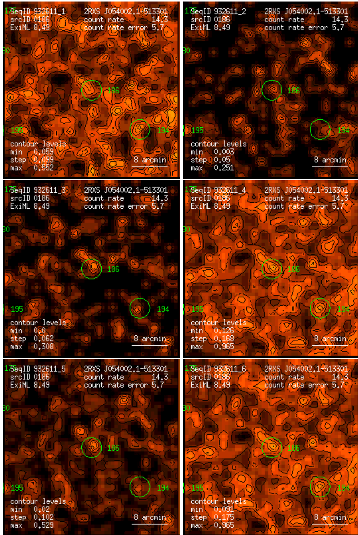
Figure 186: RASS 932611: detection 0186: band rate images, Gaussian filter: (1) PSPC channels 11 – 41, (2) 52 – 90, (3) 91 – 201, (4) 11 – 235, (5) 52 – 201, (6) 11 – 201. Broad band rates in counts/ks. Band rate contour levels in counts/ks/arcmin 2 .
