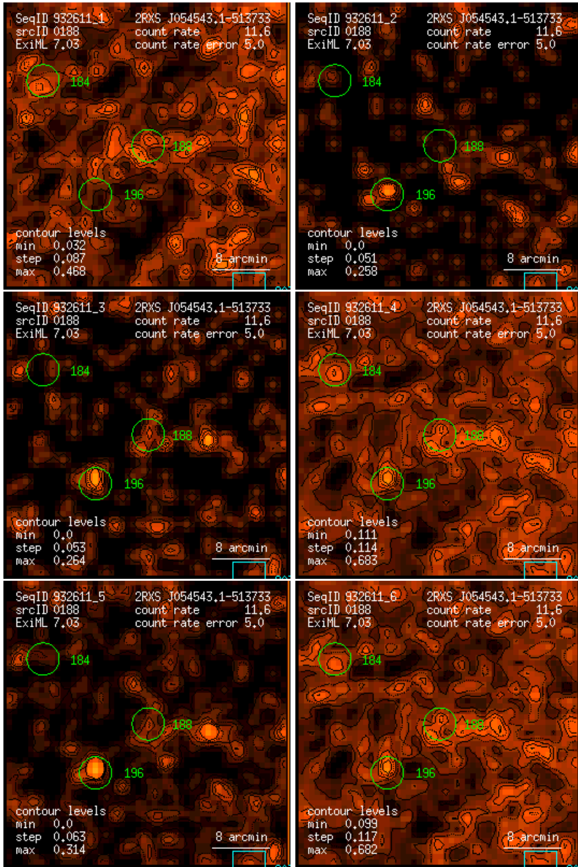
Figure 188: RASS 932611: detection 0188: band rate images, Gaussian filter: (1) PSPC channels 11 – 41, (2) 52 – 90, (3) 91 – 201, (4) 11 – 235, (5) 52 – 201, (6) 11 – 201. Broad band rates in counts/ks. Band rate contour levels in counts/ks/arcmin 2 .
