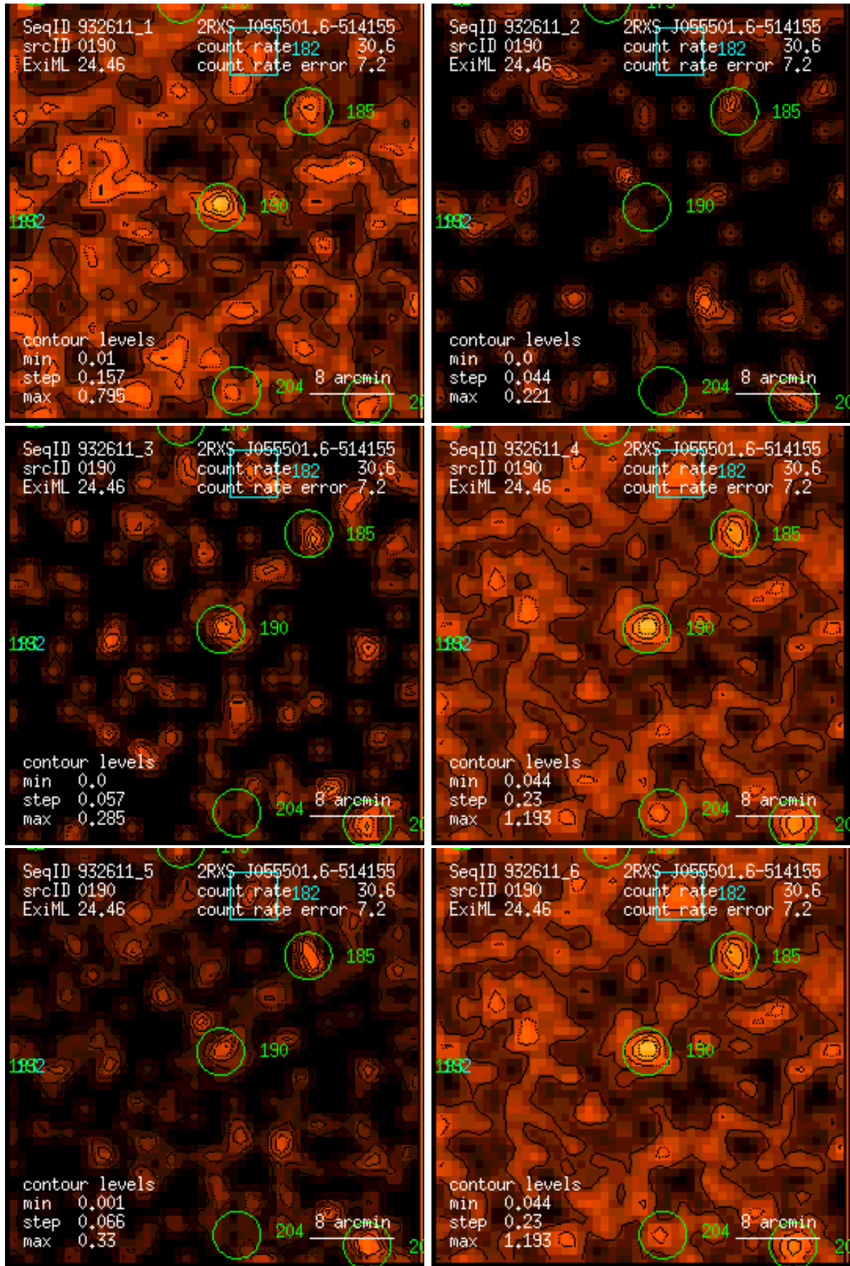
Figure 190: RASS 932611: detection 0190: band rate images, Gaussian filter: (1) PSPC channels 11 – 41, (2) 52 – 90, (3) 91 – 201, (4) 11 – 235, (5) 52 – 201, (6) 11 – 201. Broad band rates in counts/ks. Band rate contour levels in counts/ks/arcmin 2 .
