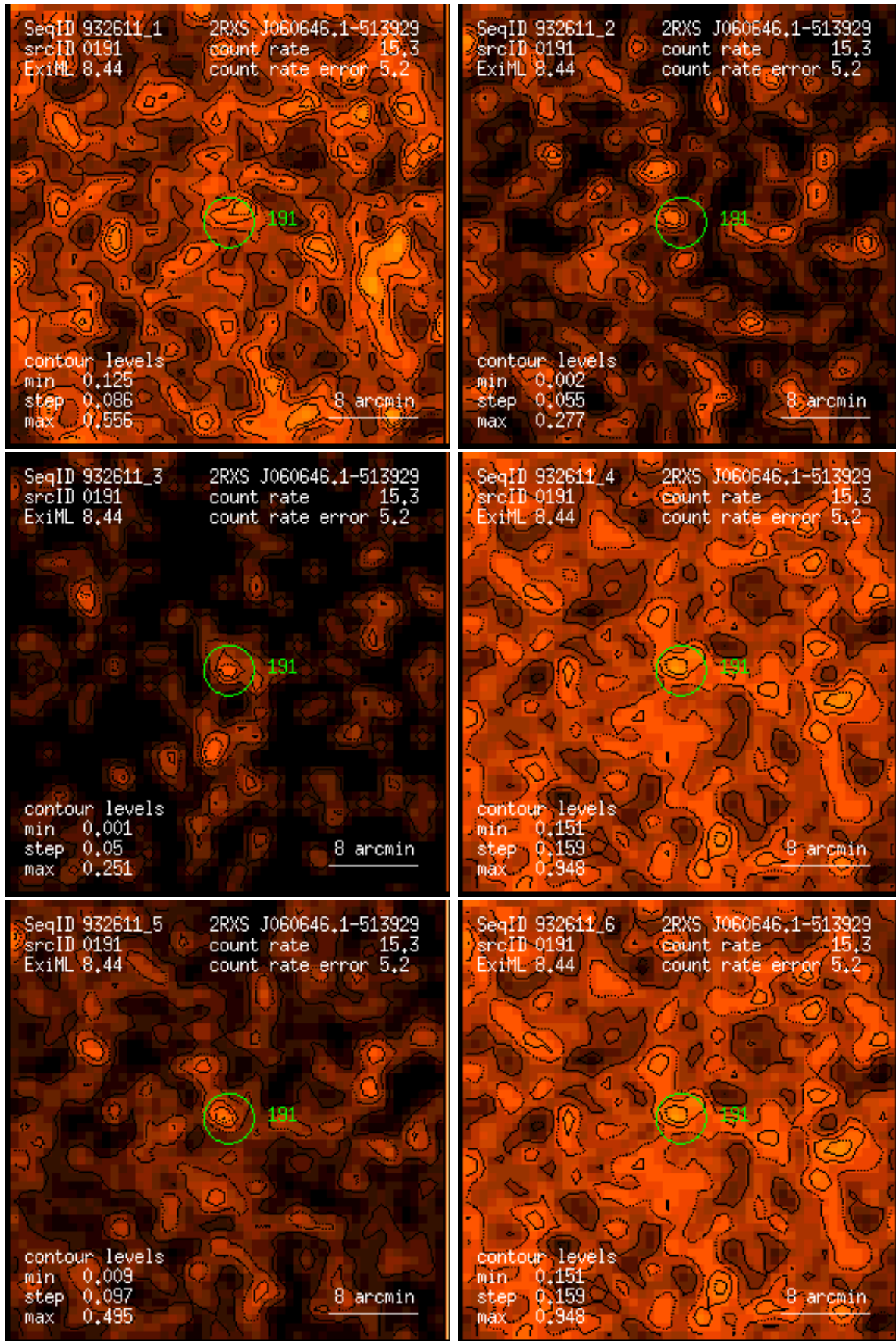
Figure 191: RASS 932611: detection 0191: band rate images, Gaussian filter: (1) PSPC channels 11 – 41, (2) 52 – 90, (3) 91 – 201, (4) 11 – 235, (5) 52 – 201, (6) 11 – 201. Broad band rates in counts/ks. Band rate contour levels in counts/ks/arcmin 2 .
