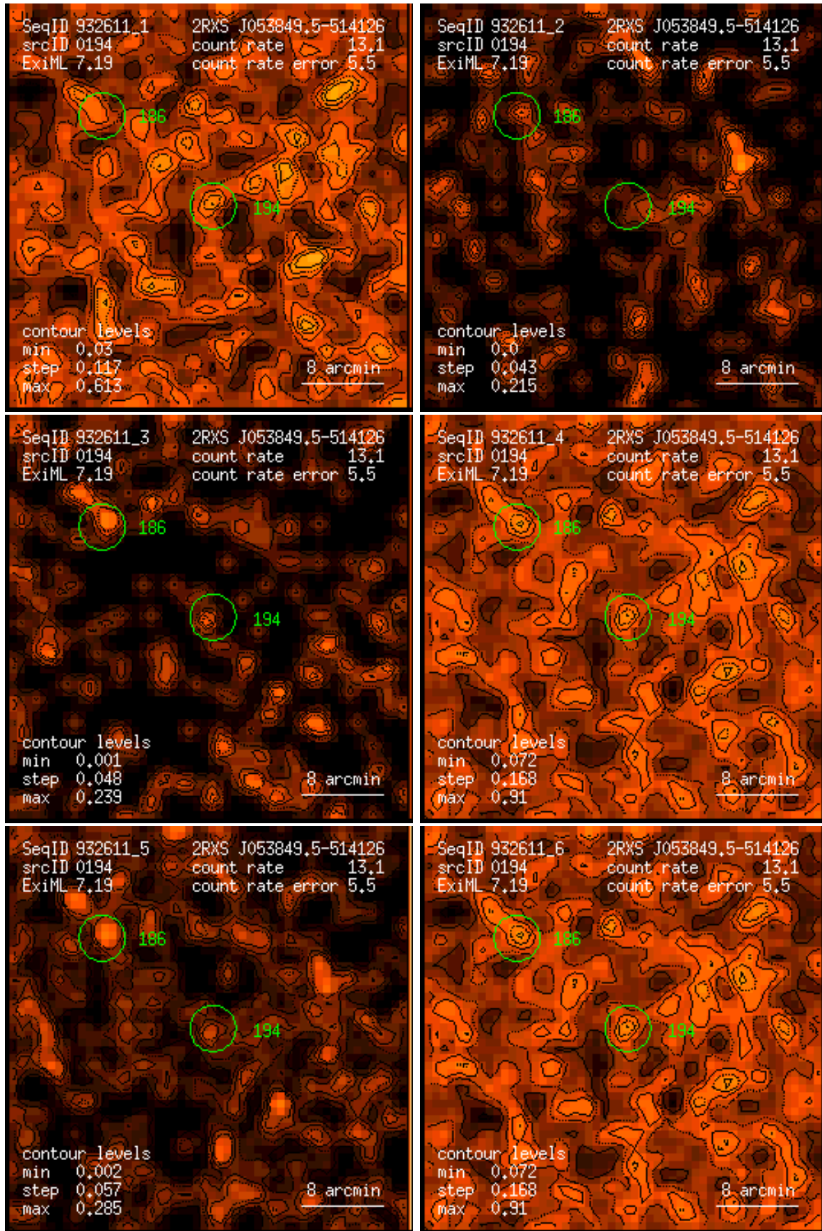
Figure 194: RASS 932611: detection 0194: band rate images, Gaussian filter: (1) PSPC channels 11 – 41, (2) 52 – 90, (3) 91 – 201, (4) 11 – 235, (5) 52 – 201, (6) 11 – 201. Broad band rates in counts/ks. Band rate contour levels in counts/ks/arcmin 2 .
