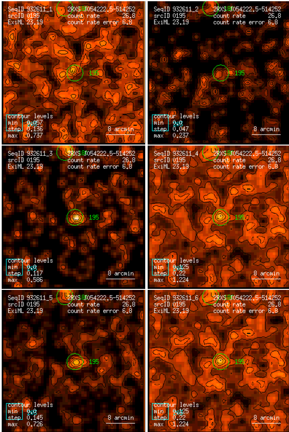
Figure 195: RASS 932611: detection 0195: band rate images, Gaussian filter: (1) PSPC channels 11 – 41, (2) 52 – 90, (3) 91 – 201, (4) 11 – 235, (5) 52 – 201, (6) 11 – 201. Broad band rates in counts/ks. Band rate contour levels in counts/ks/arcmin 2 .
