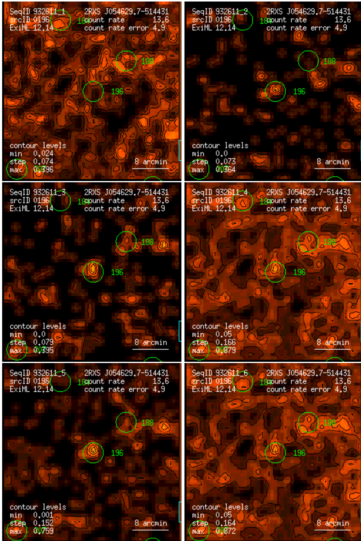
Figure 196: RASS 932611: detection 0196: band rate images, Gaussian filter: (1) PSPC channels 11 – 41, (2) 52 – 90, (3) 91 – 201, (4) 11 – 235, (5) 52 – 201, (6) 11 – 201. Broad band rates in counts/ks. Band rate contour levels in counts/ks/arcmin 2 .
