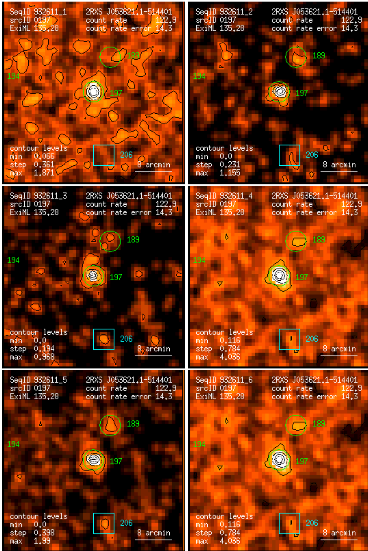
Figure 197: RASS 932611: detection 0197: band rate images, Gaussian filter: (1) PSPC channels 11 – 41, (2) 52 – 90, (3) 91 – 201, (4) 11 – 235, (5) 52 – 201, (6) 11 – 201. Broad band rates in counts/ks. Band rate contour levels in counts/ks/arcmin 2 .
