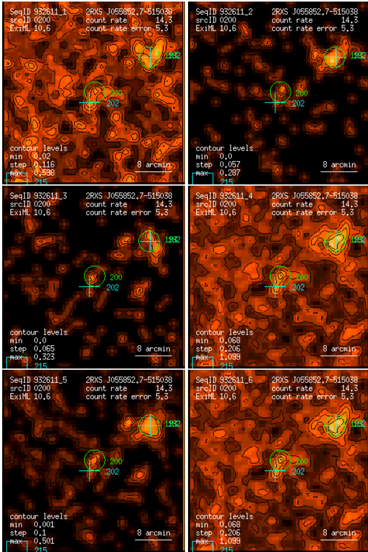
Figure 200: RASS 932611: detection 0200: band rate images, Gaussian filter: (1) PSPC channels 11 – 41, (2) 52 – 90, (3) 91 – 201, (4) 11 – 235, (5) 52 – 201, (6) 11 – 201. Broad band rates in counts/ks. Band rate contour levels in counts/ks/arcmin 2 .
