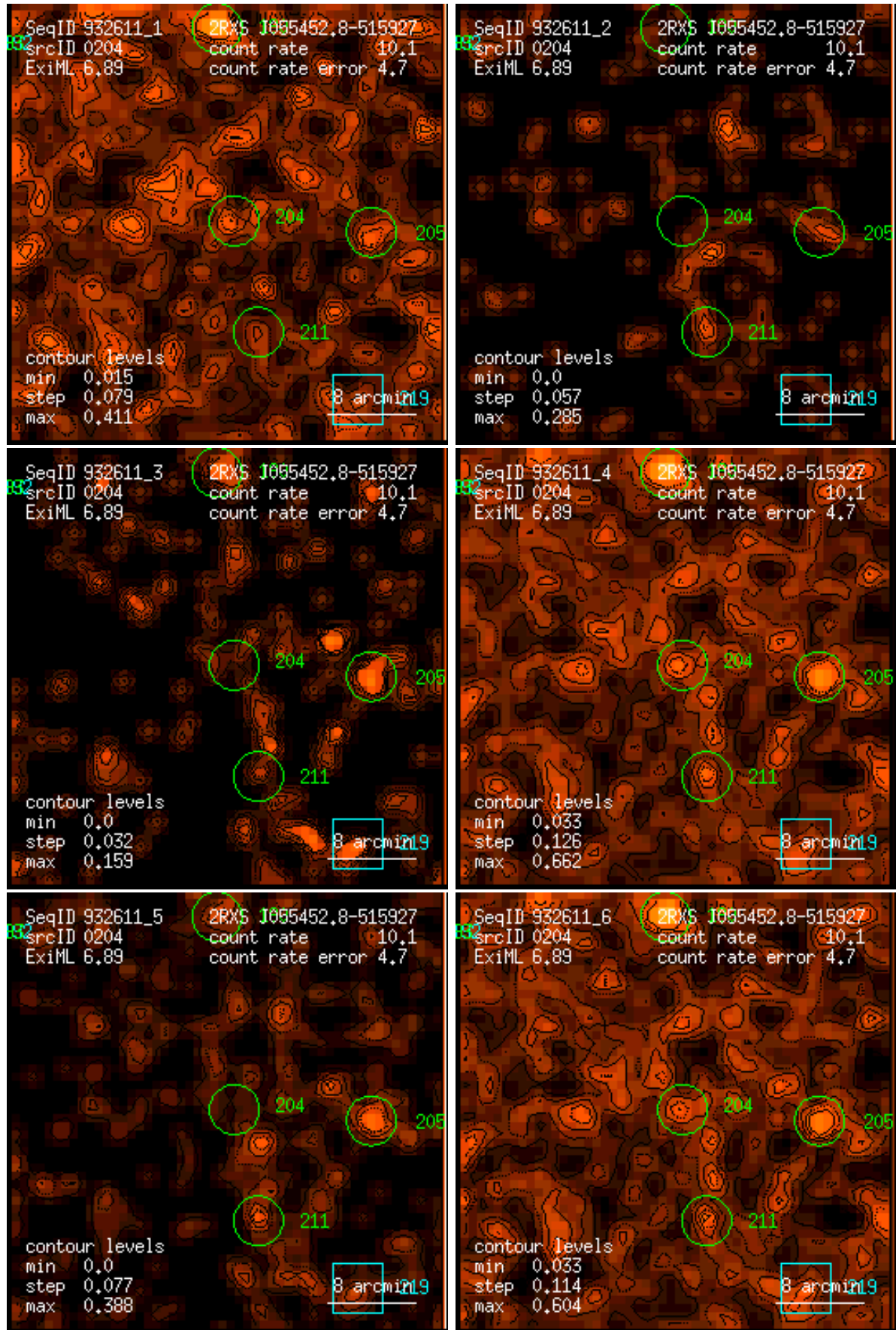
Figure 204: RASS 932611: detection 0204: band rate images, Gaussian filter: (1) PSPC channels 11 – 41, (2) 52 – 90, (3) 91 – 201, (4) 11 – 235, (5) 52 – 201, (6) 11 – 201. Broad band rates in counts/ks. Band rate contour levels in counts/ks/arcmin 2 .
