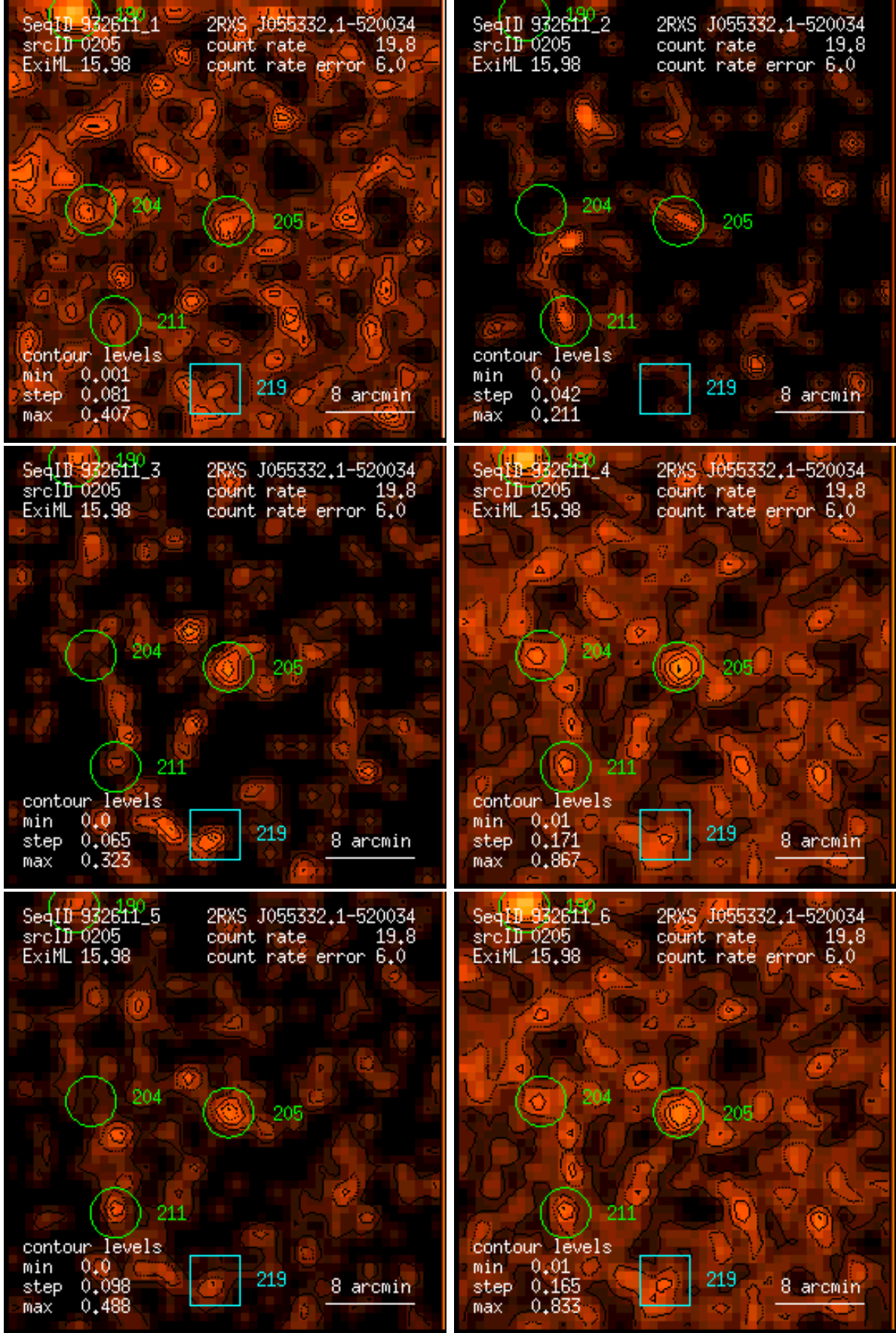
Figure 205: RASS 932611: detection 0205: band rate images, Gaussian filter: (1) PSPC channels 11 – 41, (2) 52 – 90, (3) 91 – 201, (4) 11 – 235, (5) 52 – 201, (6) 11 – 201. Broad band rates in counts/ks. Band rate contour levels in counts/ks/arcmin 2 .
