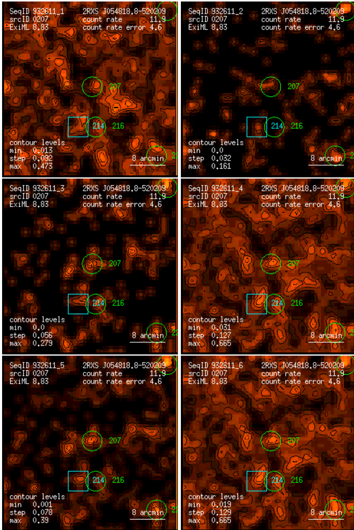
Figure 207: RASS 932611: detection 0207: band rate images, Gaussian filter: (1) PSPC channels 11 – 41, (2) 52 – 90, (3) 91 – 201, (4) 11 – 235, (5) 52 – 201, (6) 11 – 201. Broad band rates in counts/ks. Band rate contour levels in counts/ks/arcmin 2 .
