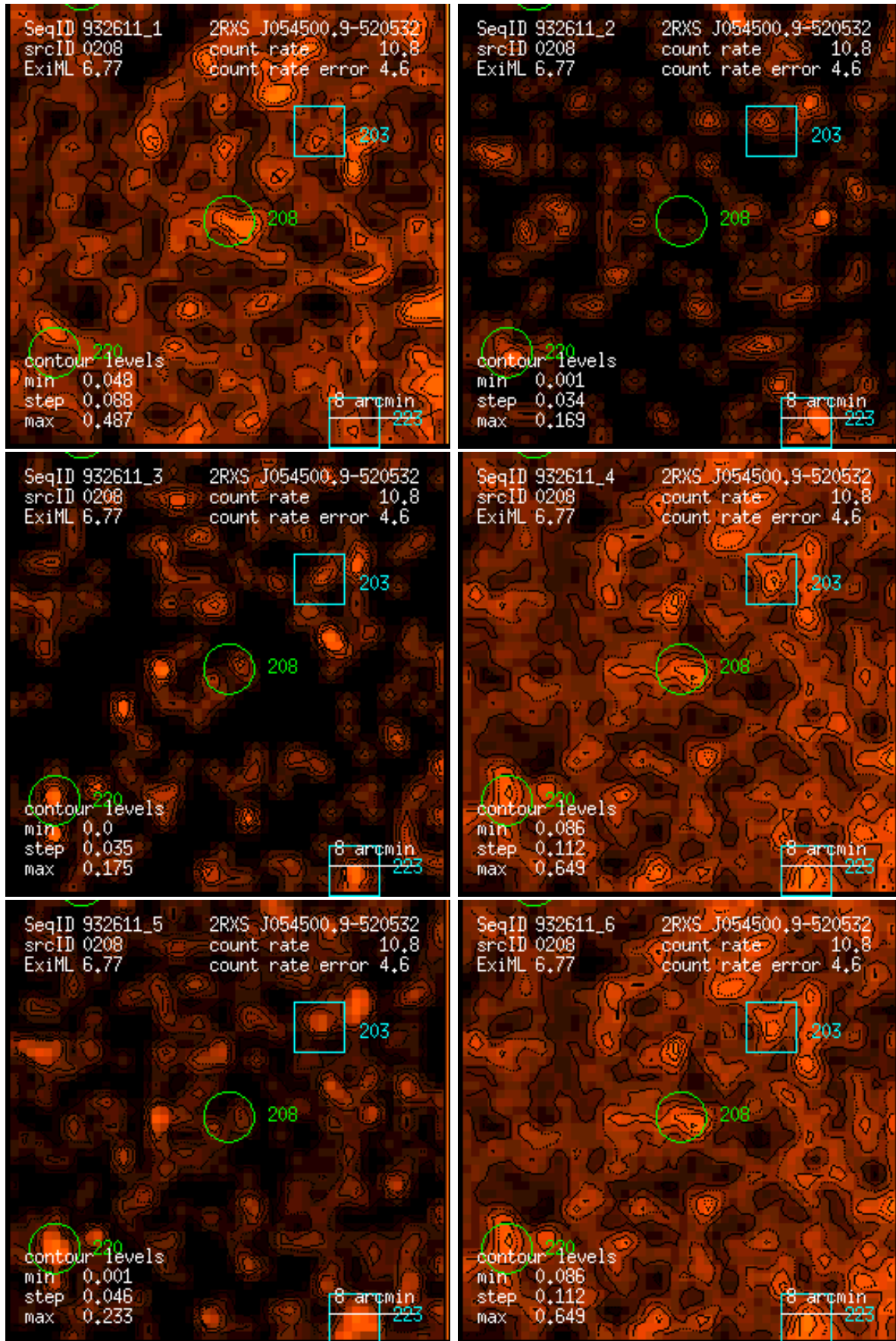
Figure 208: RASS 932611: detection 0208: band rate images, Gaussian filter: (1) PSPC channels 11 – 41, (2) 52 – 90, (3) 91 – 201, (4) 11 – 235, (5) 52 – 201, (6) 11 – 201. Broad band rates in counts/ks. Band rate contour levels in counts/ks/arcmin 2 .
