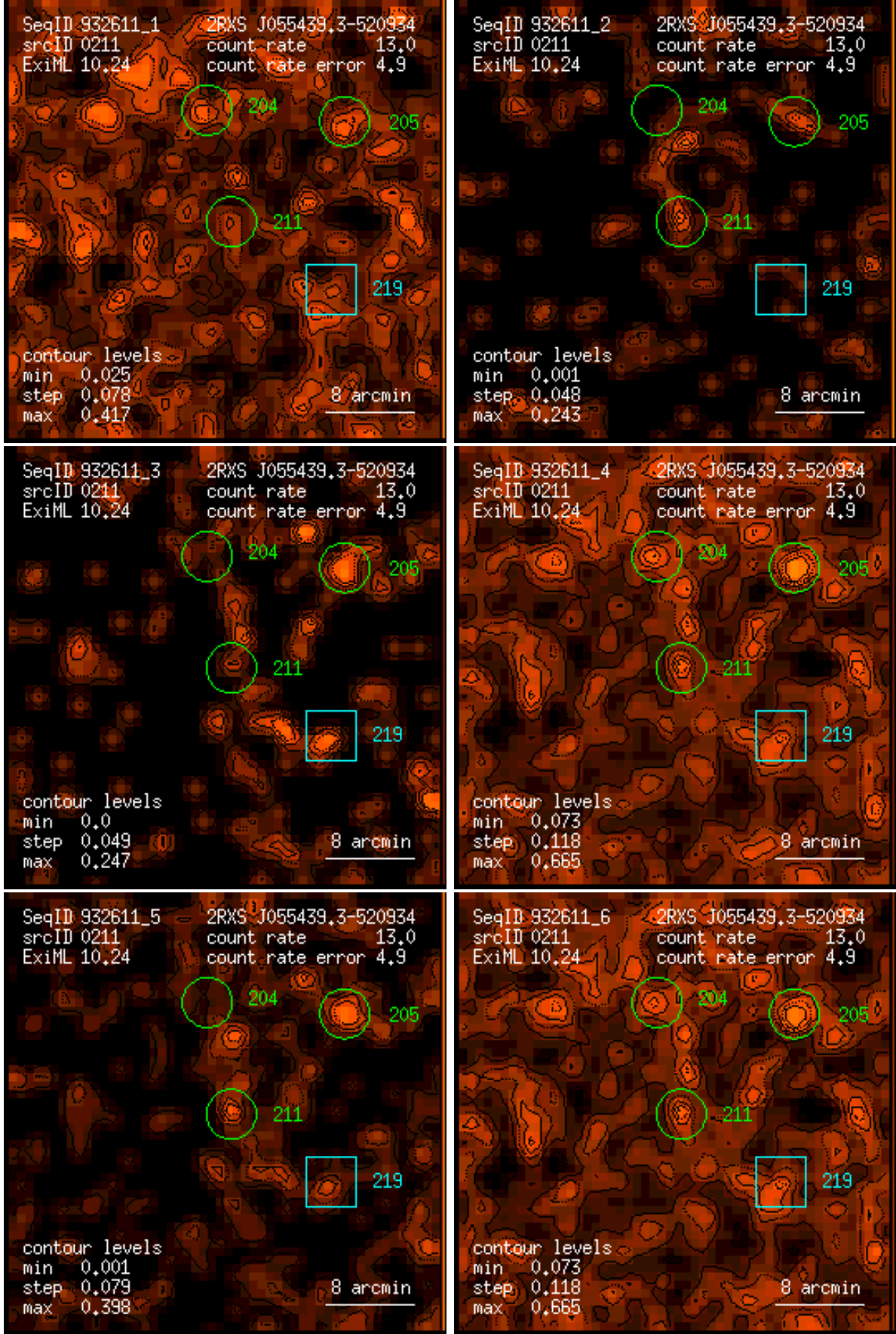
Figure 211: RASS 932611: detection 0211: band rate images, Gaussian filter: (1) PSPC channels 11 – 41, (2) 52 – 90, (3) 91 – 201, (4) 11 – 235, (5) 52 – 201, (6) 11 – 201. Broad band rates in counts/ks. Band rate contour levels in counts/ks/arcmin 2 .
