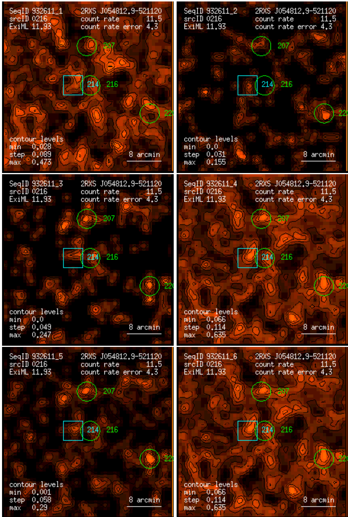
Figure 216: RASS 932611: detection 0216: band rate images, Gaussian filter: (1) PSPC channels 11 – 41, (2) 52 – 90, (3) 91 – 201, (4) 11 – 235, (5) 52 – 201, (6) 11 – 201. Broad band rates in counts/ks. Band rate contour levels in counts/ks/arcmin 2 .
