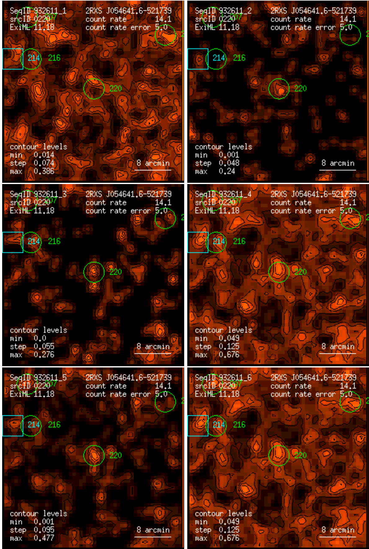
Figure 220: RASS 932611: detection 0220: band rate images, Gaussian filter: (1) PSPC channels 11 – 41, (2) 52 – 90, (3) 91 – 201, (4) 11 – 235, (5) 52 – 201, (6) 11 – 201. Broad band rates in counts/ks. Band rate contour levels in counts/ks/arcmin 2 .
