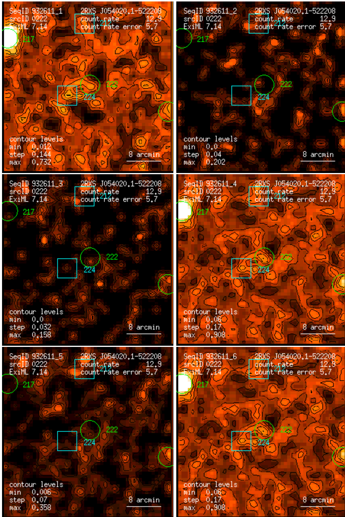
Figure 222: RASS 932611: detection 0222: band rate images, Gaussian filter: (1) PSPC channels 11 – 41, (2) 52 – 90, (3) 91 – 201, (4) 11 – 235, (5) 52 – 201, (6) 11 – 201. Broad band rates in counts/ks. Band rate contour levels in counts/ks/arcmin 2 .
