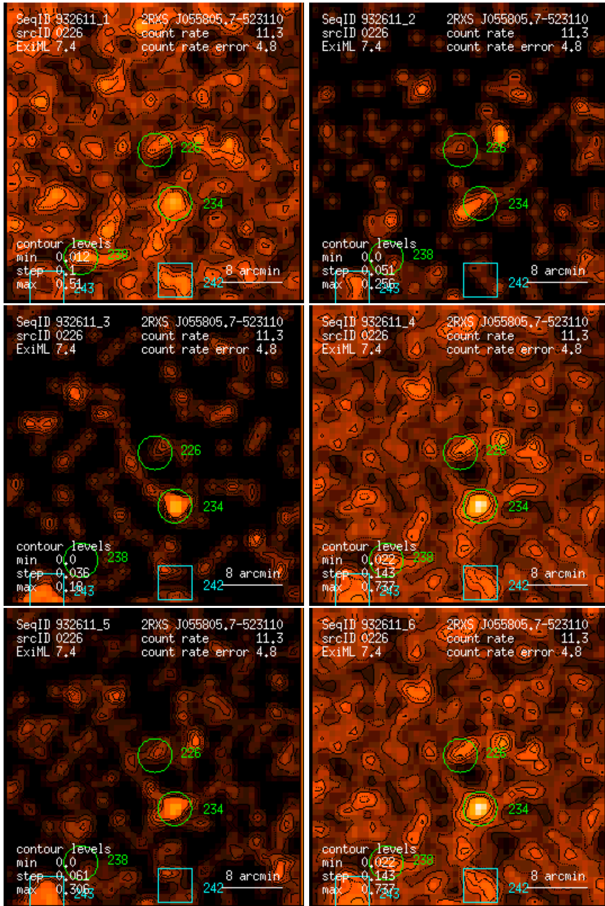
Figure 226: RASS 932611: detection 0226: band rate images, Gaussian filter: (1) PSPC channels 11 – 41, (2) 52 – 90, (3) 91 – 201, (4) 11 – 235, (5) 52 – 201, (6) 11 – 201. Broad band rates in counts/ks. Band rate contour levels in counts/ks/arcmin 2 .
