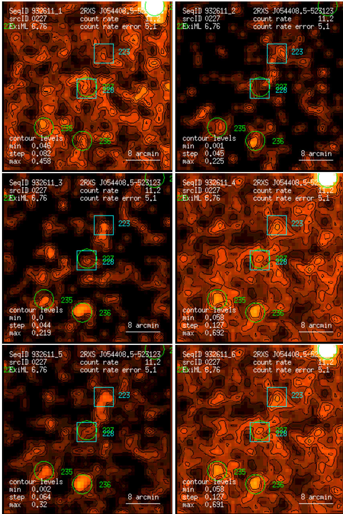
Figure 227: RASS 932611: detection 0227: band rate images, Gaussian filter: (1) PSPC channels 11 – 41, (2) 52 – 90, (3) 91 – 201, (4) 11 – 235, (5) 52 – 201, (6) 11 – 201. Broad band rates in counts/ks. Band rate contour levels in counts/ks/arcmin 2 .
