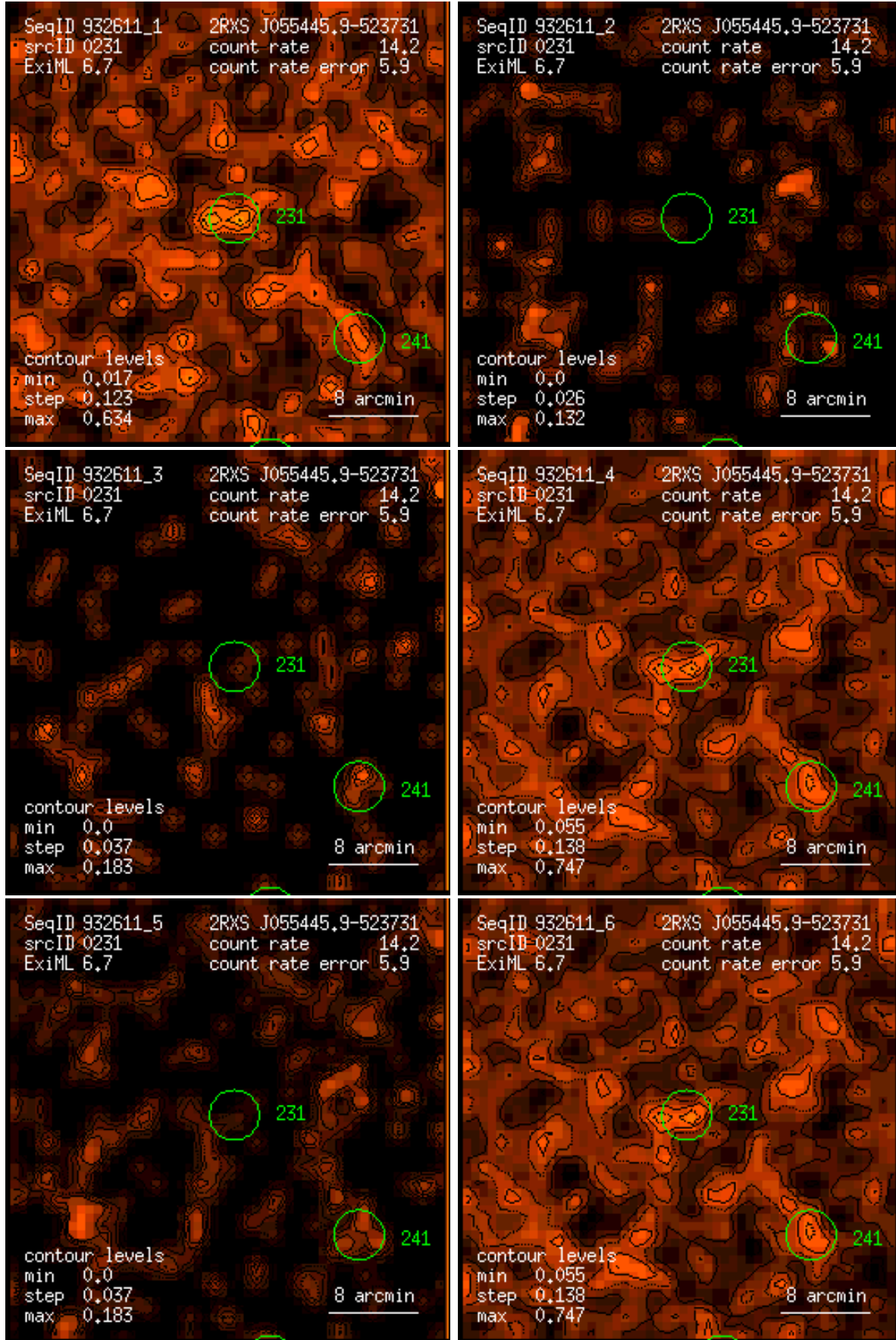
Figure 231: RASS 932611: detection 0231: band rate images, Gaussian filter: (1) PSPC channels 11 – 41, (2) 52 – 90, (3) 91 – 201, (4) 11 – 235, (5) 52 – 201, (6) 11 – 201. Broad band rates in counts/ks. Band rate contour levels in counts/ks/arcmin 2 .
