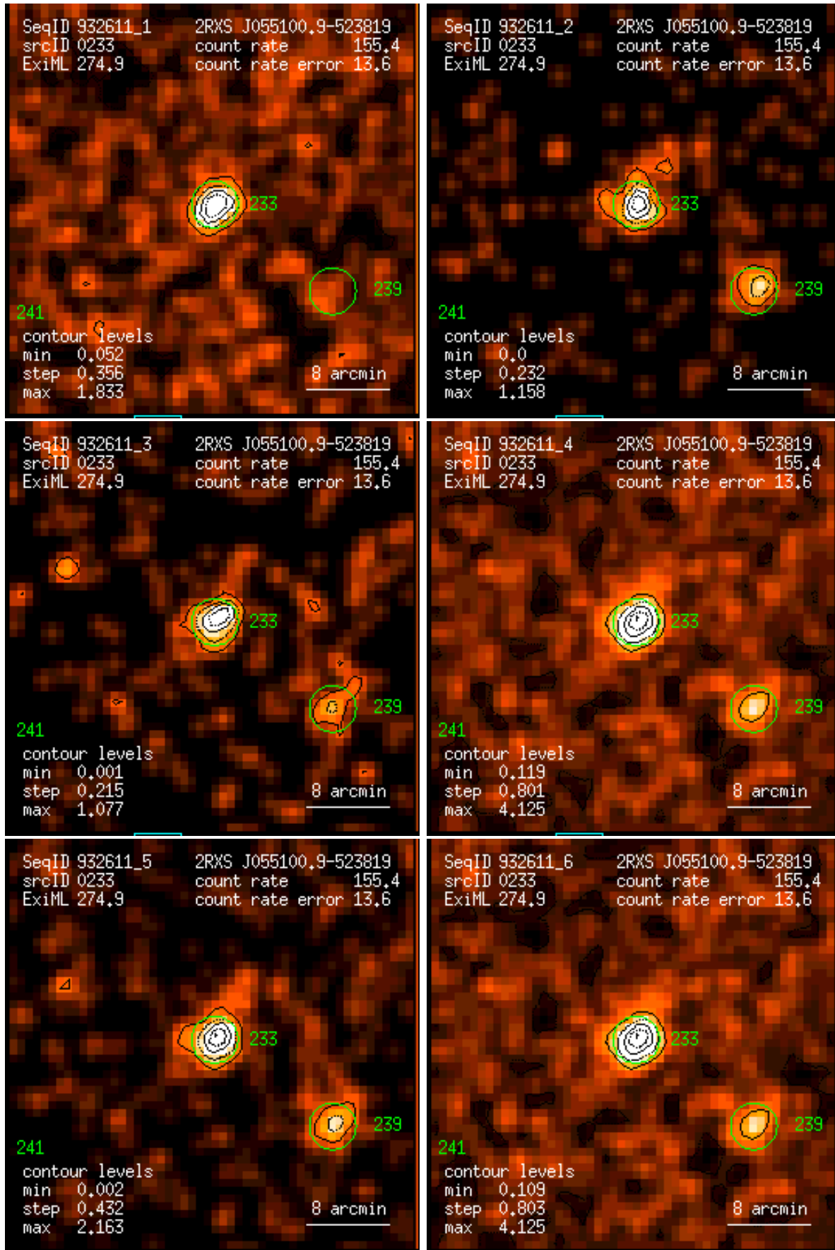
Figure 233: RASS 932611: detection 0233: band rate images, Gaussian filter: (1) PSPC channels 11 – 41, (2) 52 – 90, (3) 91 – 201, (4) 11 – 235, (5) 52 – 201, (6) 11 – 201. Broad band rates in counts/ks. Band rate contour levels in counts/ks/arcmin 2 .
