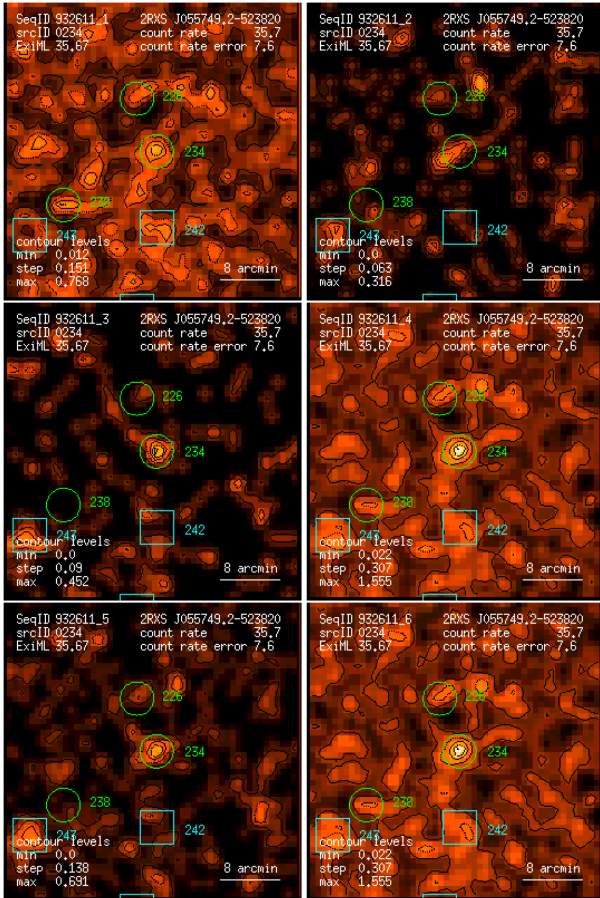
Figure 234: RASS 932611: detection 0234: band rate images, Gaussian filter: (1) PSPC channels 11 – 41, (2) 52 – 90, (3) 91 – 201, (4) 11 – 235, (5) 52 – 201, (6) 11 – 201. Broad band rates in counts/ks. Band rate contour levels in counts/ks/arcmin 2 .
