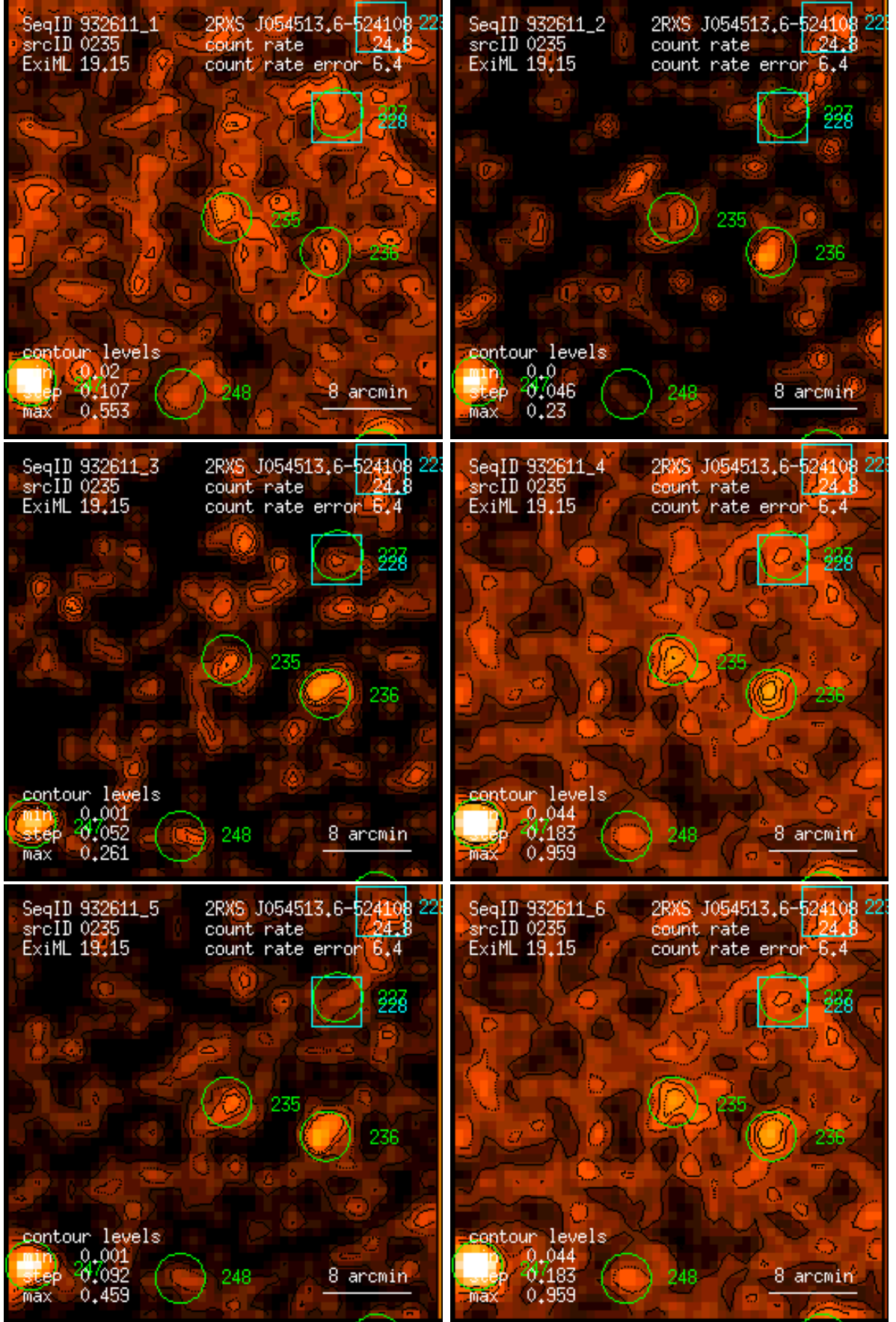
Figure 235: RASS 932611: detection 0235: band rate images, Gaussian filter: (1) PSPC channels 11 – 41, (2) 52 – 90, (3) 91 – 201, (4) 11 – 235, (5) 52 – 201, (6) 11 – 201. Broad band rates in counts/ks. Band rate contour levels in counts/ks/arcmin 2 .
