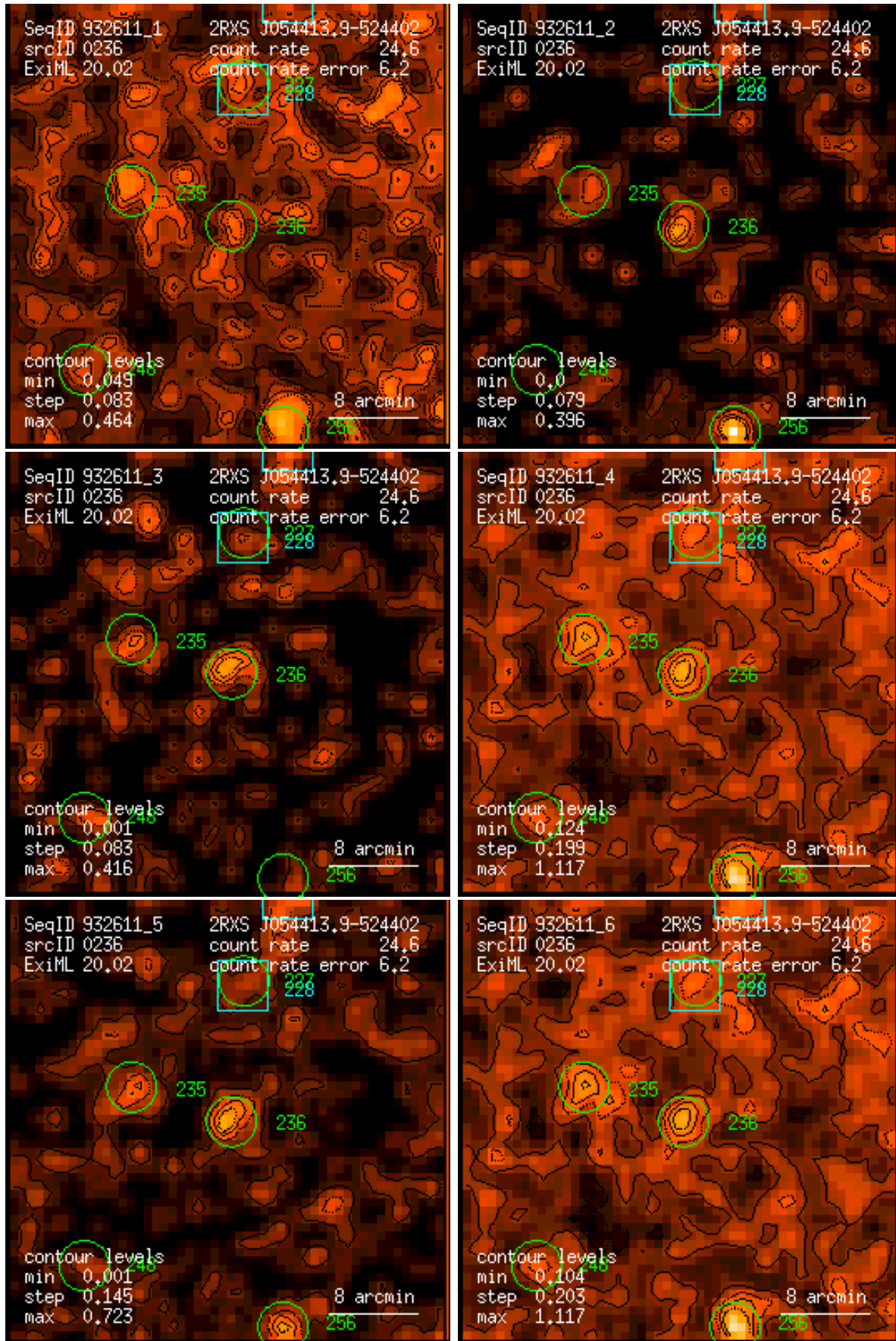
Figure 236: RASS 932611: detection 0236: band rate images, Gaussian filter: (1) PSPC channels 11 – 41, (2) 52 – 90, (3) 91 – 201, (4) 11 – 235, (5) 52 – 201, (6) 11 – 201. Broad band rates in counts/ks. Band rate contour levels in counts/ks/arcmin 2 .
