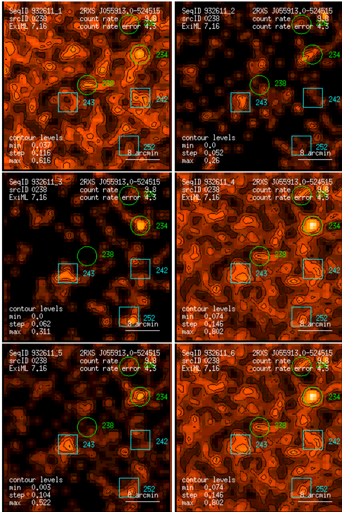
Figure 238: RASS 932611: detection 0238: band rate images, Gaussian filter: (1) PSPC channels 11 – 41, (2) 52 – 90, (3) 91 – 201, (4) 11 – 235, (5) 52 – 201, (6) 11 – 201. Broad band rates in counts/ks. Band rate contour levels in counts/ks/arcmin 2 .
