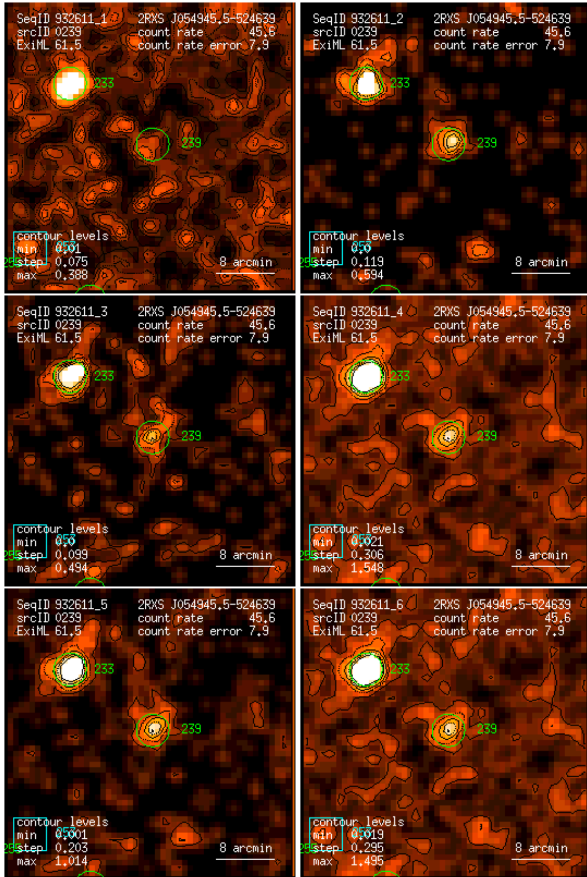
Figure 239: RASS 932611: detection 0239: band rate images, Gaussian filter: (1) PSPC channels 11 – 41, (2) 52 – 90, (3) 91 – 201, (4) 11 – 235, (5) 52 – 201, (6) 11 – 201. Broad band rates in counts/ks. Band rate contour levels in counts/ks/arcmin 2 .
