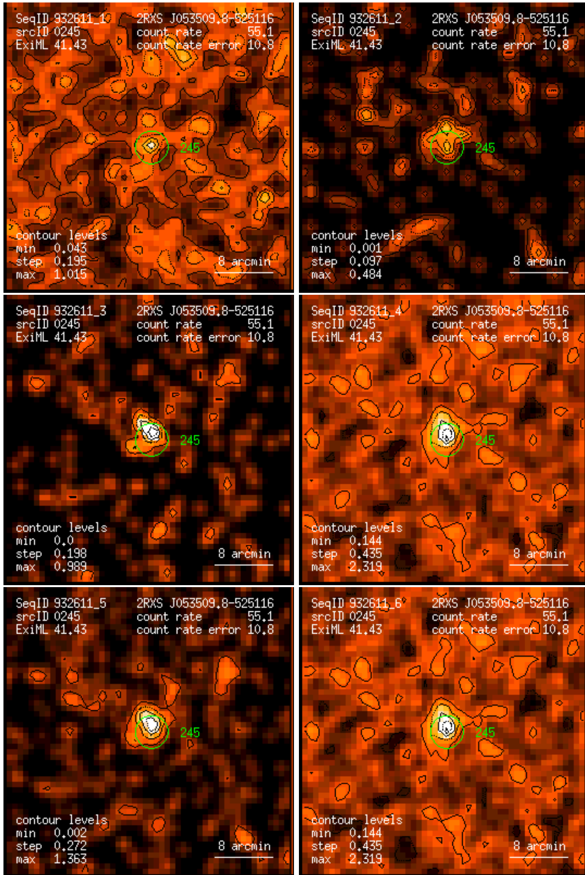
Figure 245: RASS 932611: detection 0245: band rate images, Gaussian filter: (1) PSPC channels 11 – 41, (2) 52 – 90, (3) 91 – 201, (4) 11 – 235, (5) 52 – 201, (6) 11 – 201. Broad band rates in counts/ks. Band rate contour levels in counts/ks/arcmin 2 .
