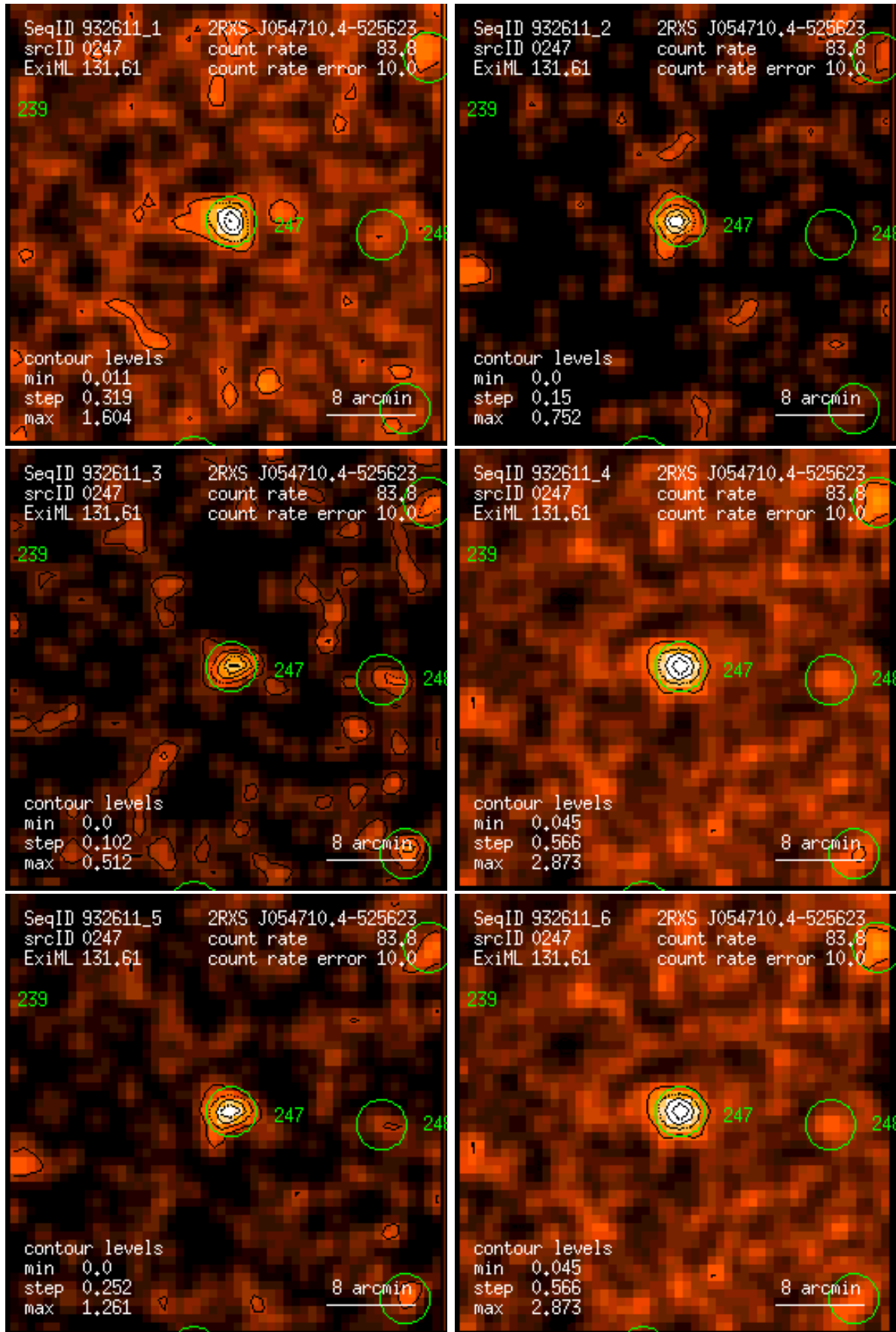
Figure 247: RASS 932611: detection 0247: band rate images, Gaussian filter: (1) PSPC channels 11 – 41, (2) 52 – 90, (3) 91 – 201, (4) 11 – 235, (5) 52 – 201, (6) 11 – 201. Broad band rates in counts/ks. Band rate contour levels in counts/ks/arcmin 2 .
