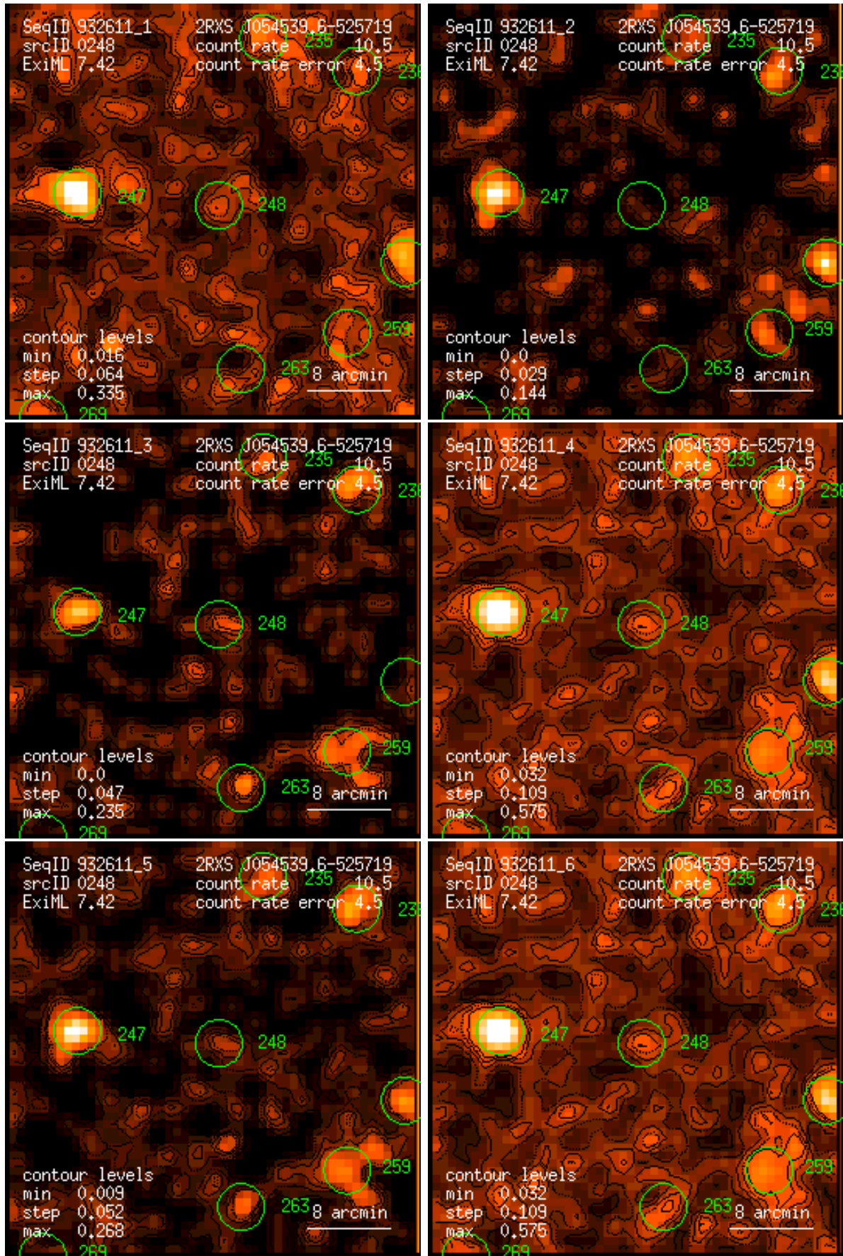
Figure 248: RASS 932611: detection 0248: band rate images, Gaussian filter: (1) PSPC channels 11 – 41, (2) 52 – 90, (3) 91 – 201, (4) 11 – 235, (5) 52 – 201, (6) 11 – 201. Broad band rates in counts/ks. Band rate contour levels in counts/ks/arcmin 2 .
