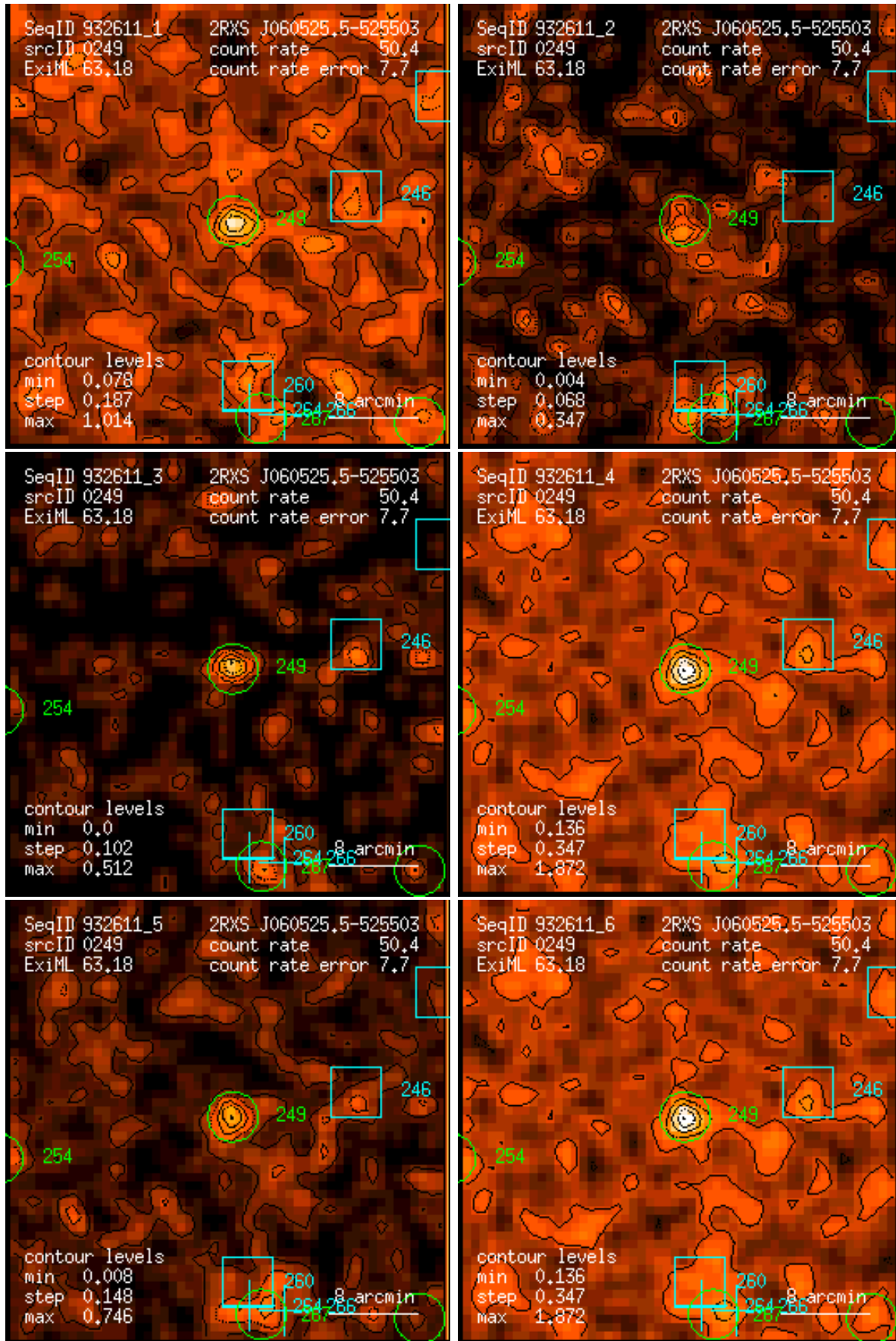
Figure 249: RASS 932611: detection 0249: band rate images, Gaussian filter: (1) PSPC channels 11 – 41, (2) 52 – 90, (3) 91 – 201, (4) 11 – 235, (5) 52 – 201, (6) 11 – 201. Broad band rates in counts/ks. Band rate contour levels in counts/ks/arcmin 2 .
