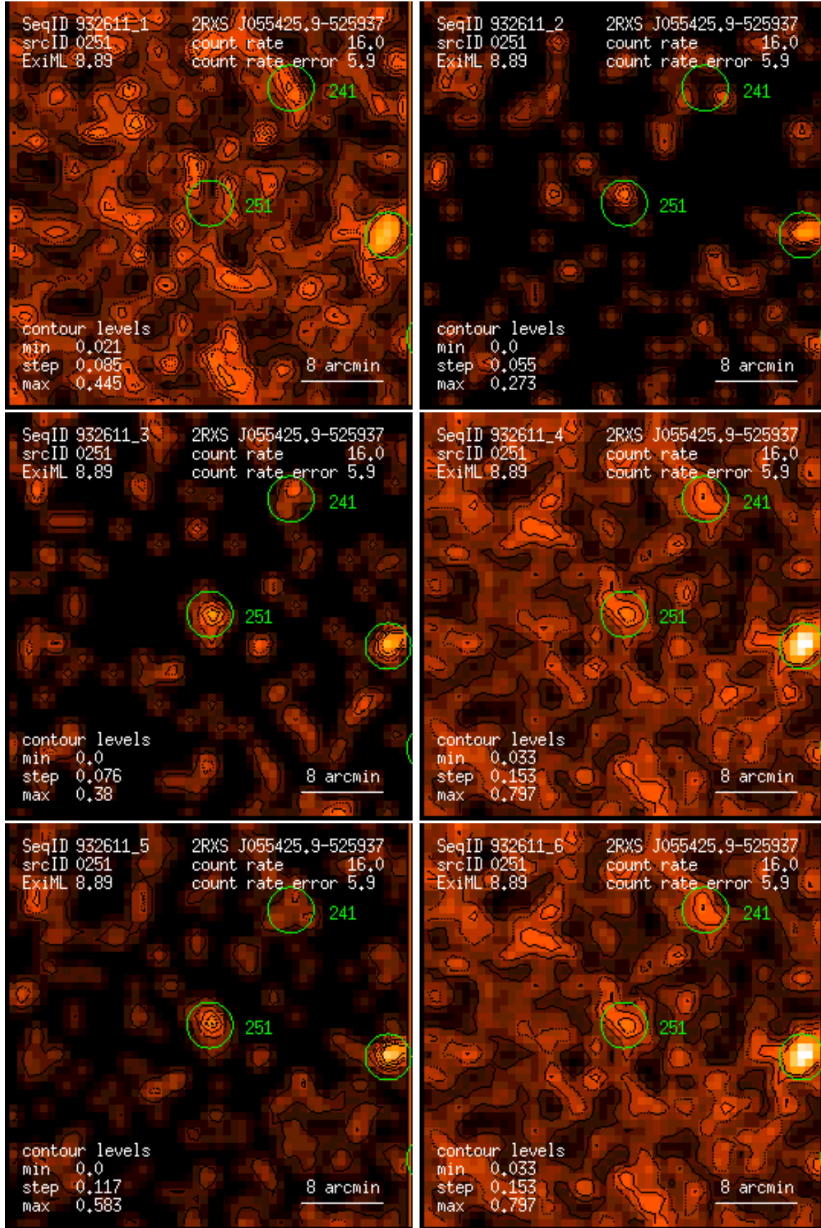
Figure 251: RASS 932611: detection 0251: band rate images, Gaussian filter: (1) PSPC channels 11 – 41, (2) 52 – 90, (3) 91 – 201, (4) 11 – 235, (5) 52 – 201, (6) 11 – 201. Broad band rates in counts/ks. Band rate contour levels in counts/ks/arcmin 2 .
