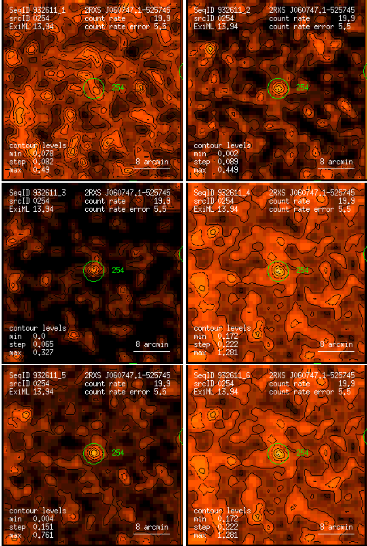
Figure 254: RASS 932611: detection 0254: band rate images, Gaussian filter: (1) PSPC channels 11 – 41, (2) 52 – 90, (3) 91 – 201, (4) 11 – 235, (5) 52 – 201, (6) 11 – 201. Broad band rates in counts/ks. Band rate contour levels in counts/ks/arcmin 2 .
