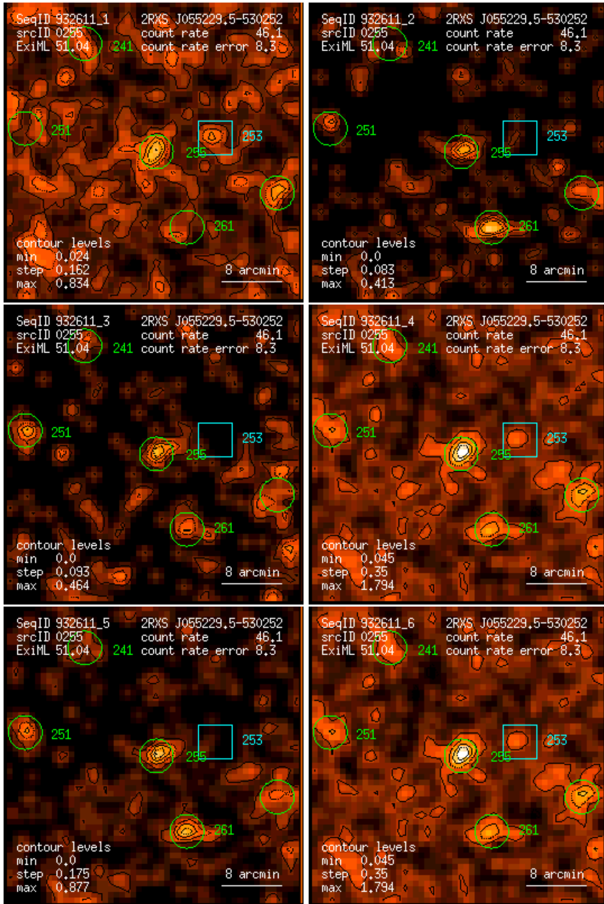
Figure 255: RASS 932611: detection 0255: band rate images, Gaussian filter: (1) PSPC channels 11 – 41, (2) 52 – 90, (3) 91 – 201, (4) 11 – 235, (5) 52 – 201, (6) 11 – 201. Broad band rates in counts/ks. Band rate contour levels in counts/ks/arcmin 2 .
