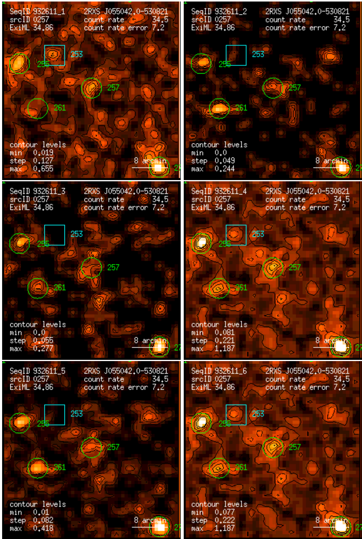
Figure 257: RASS 932611: detection 0257: band rate images, Gaussian filter: (1) PSPC channels 11 – 41, (2) 52 – 90, (3) 91 – 201, (4) 11 – 235, (5) 52 – 201, (6) 11 – 201. Broad band rates in counts/ks. Band rate contour levels in counts/ks/arcmin 2 .
