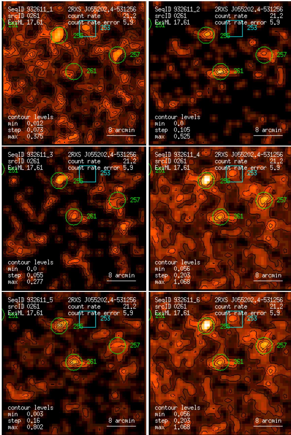
Figure 261: RASS 932611: detection 0261: band rate images, Gaussian filter: (1) PSPC channels 11 – 41, (2) 52 – 90, (3) 91 – 201, (4) 11 – 235, (5) 52 – 201, (6) 11 – 201. Broad band rates in counts/ks. Band rate contour levels in counts/ks/arcmin 2 .
