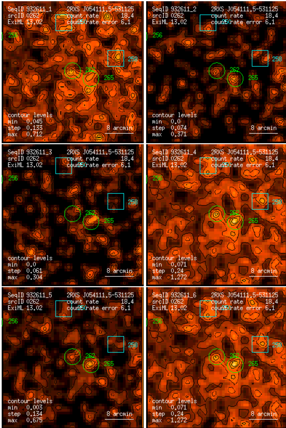
Figure 262: RASS 932611: detection 0262: band rate images, Gaussian filter: (1) PSPC channels 11 – 41, (2) 52 – 90, (3) 91 – 201, (4) 11 – 235, (5) 52 – 201, (6) 11 – 201. Broad band rates in counts/ks. Band rate contour levels in counts/ks/arcmin 2 .
