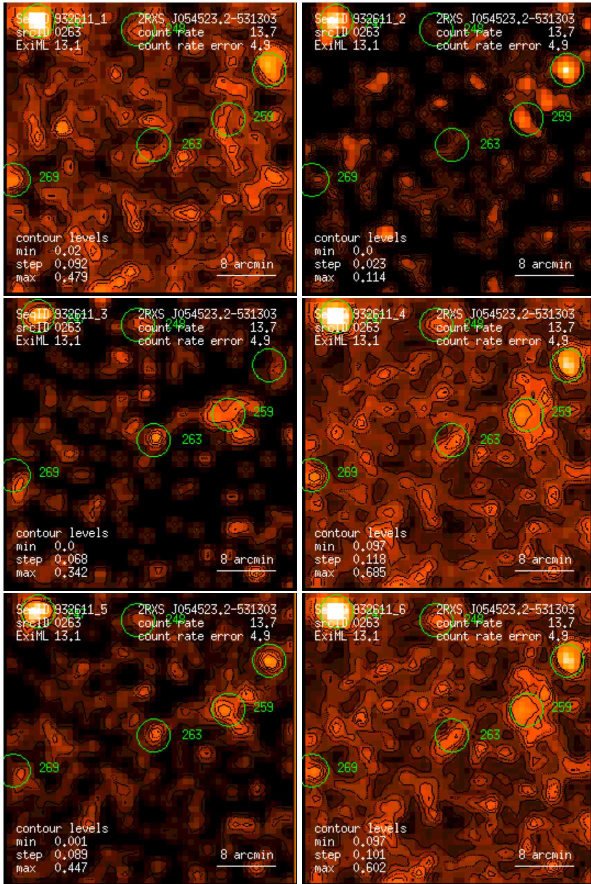
Figure 263: RASS 932611: detection 0263: band rate images, Gaussian filter: (1) PSPC channels 11 – 41, (2) 52 – 90, (3) 91 – 201, (4) 11 – 235, (5) 52 – 201, (6) 11 – 201. Broad band rates in counts/ks. Band rate contour levels in counts/ks/arcmin 2 .
