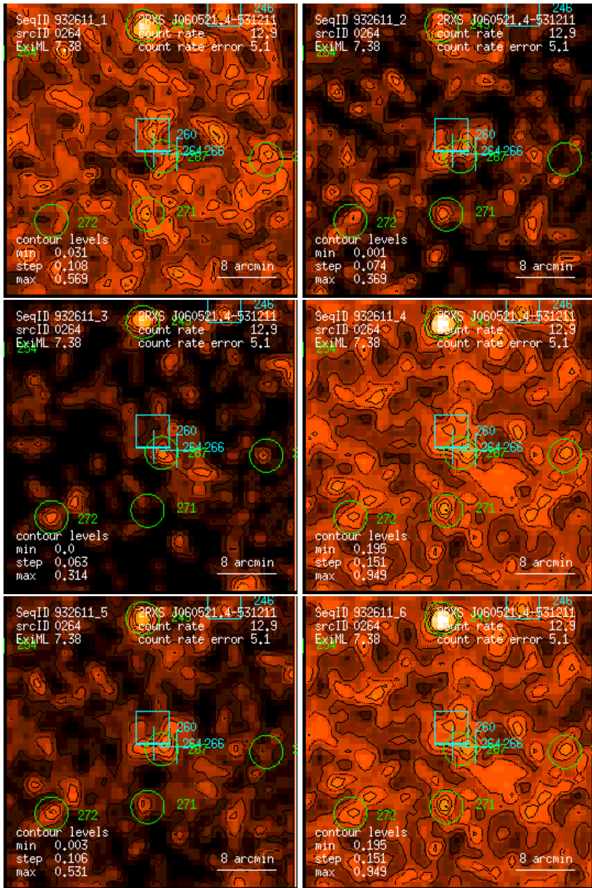
Figure 264: RASS 932611: detection 0264: band rate images, Gaussian filter: (1) PSPC channels 11 – 41, (2) 52 – 90, (3) 91 – 201, (4) 11 – 235, (5) 52 – 201, (6) 11 – 201. Broad band rates in counts/ks. Band rate contour levels in counts/ks/arcmin 2 .
