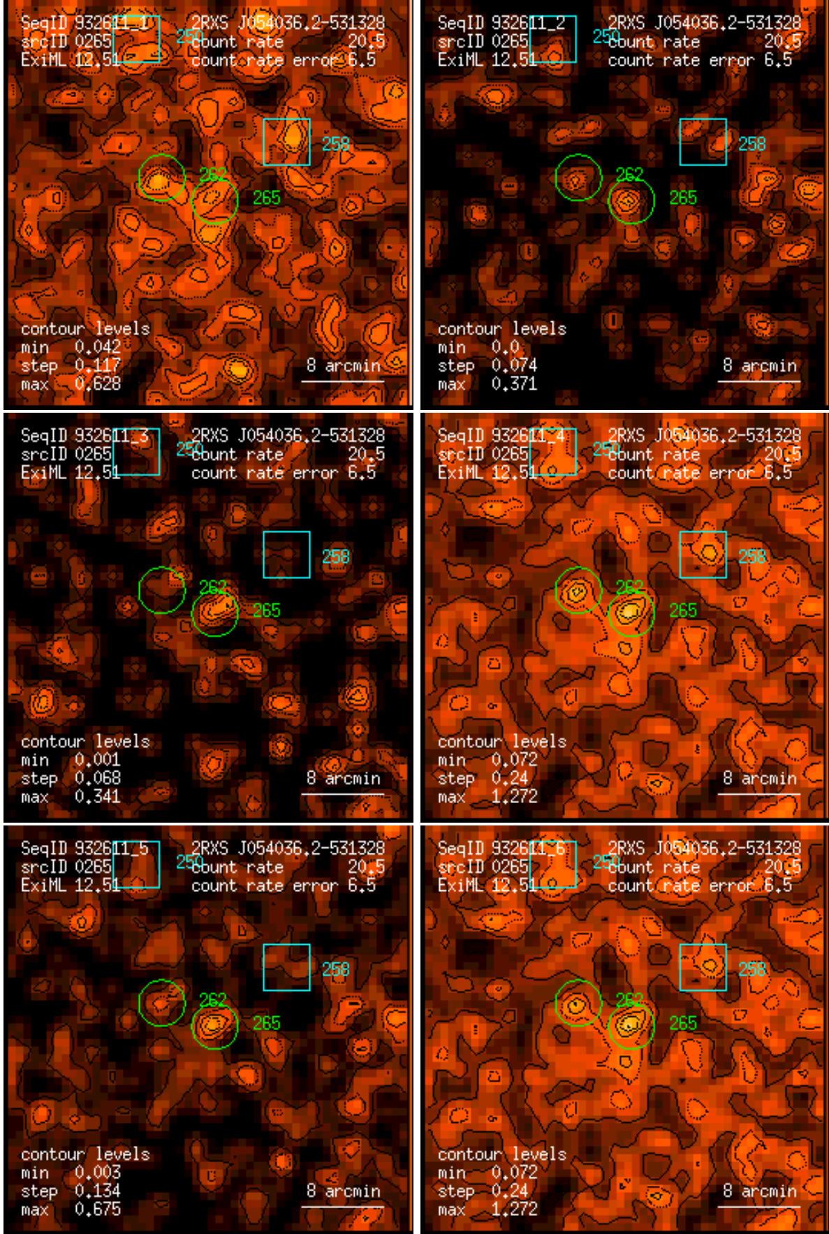
Figure 265: RASS 932611: detection 0265: band rate images, Gaussian filter: (1) PSPC channels 11 – 41, (2) 52 – 90, (3) 91 – 201, (4) 11 – 235, (5) 52 – 201, (6) 11 – 201. Broad band rates in counts/ks. Band rate contour levels in counts/ks/arcmin 2 .
