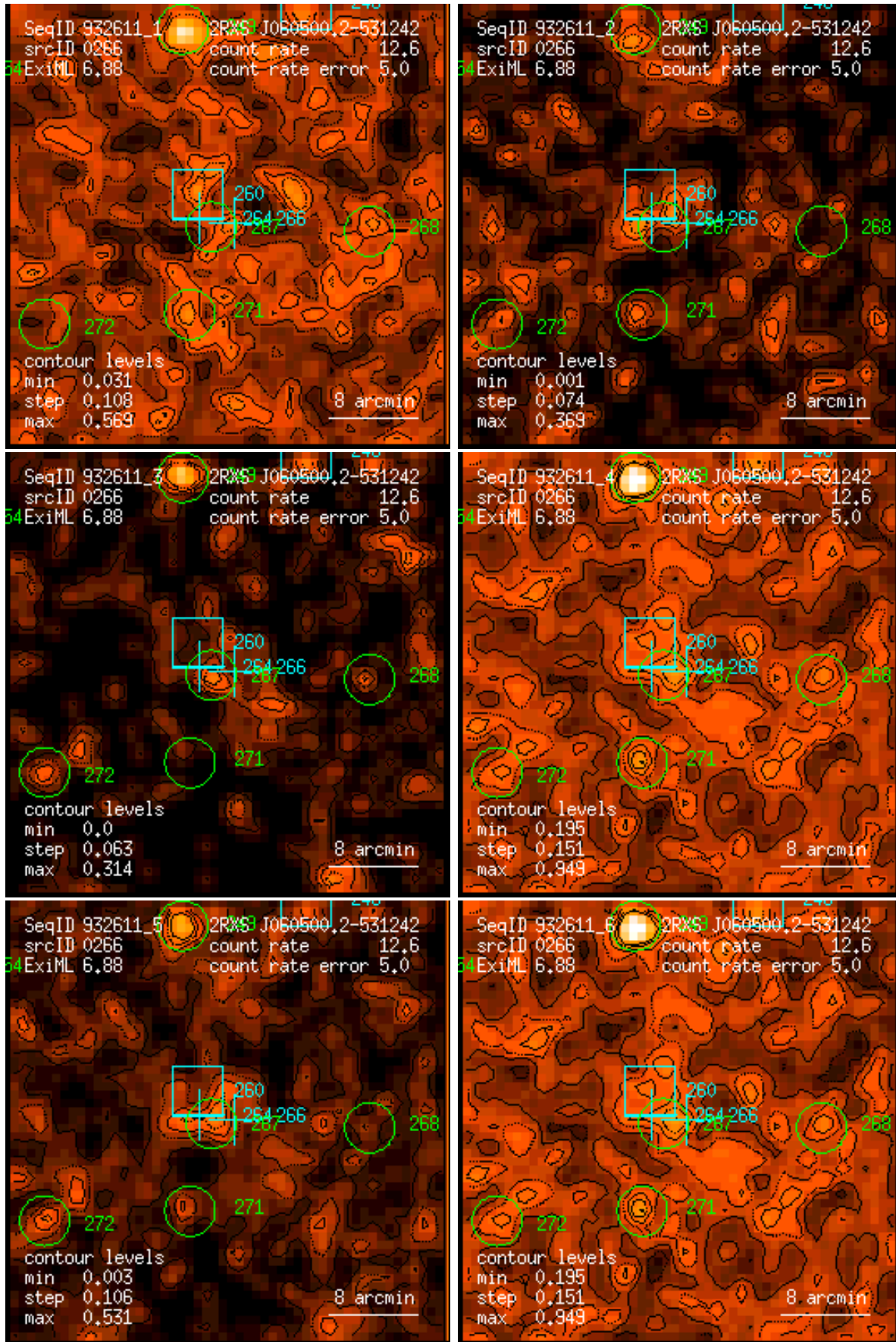
Figure 266: RASS 932611: detection 0266: band rate images, Gaussian filter: (1) PSPC channels 11 – 41, (2) 52 – 90, (3) 91 – 201, (4) 11 – 235, (5) 52 – 201, (6) 11 – 201. Broad band rates in counts/ks. Band rate contour levels in counts/ks/arcmin 2 .
