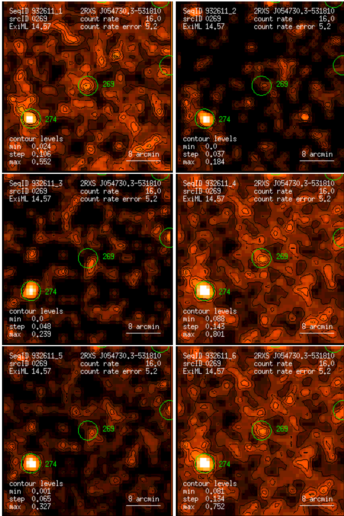
Figure 269: RASS 932611: detection 0269: band rate images, Gaussian filter: (1) PSPC channels 11 – 41, (2) 52 – 90, (3) 91 – 201, (4) 11 – 235, (5) 52 – 201, (6) 11 – 201. Broad band rates in counts/ks. Band rate contour levels in counts/ks/arcmin 2 .
