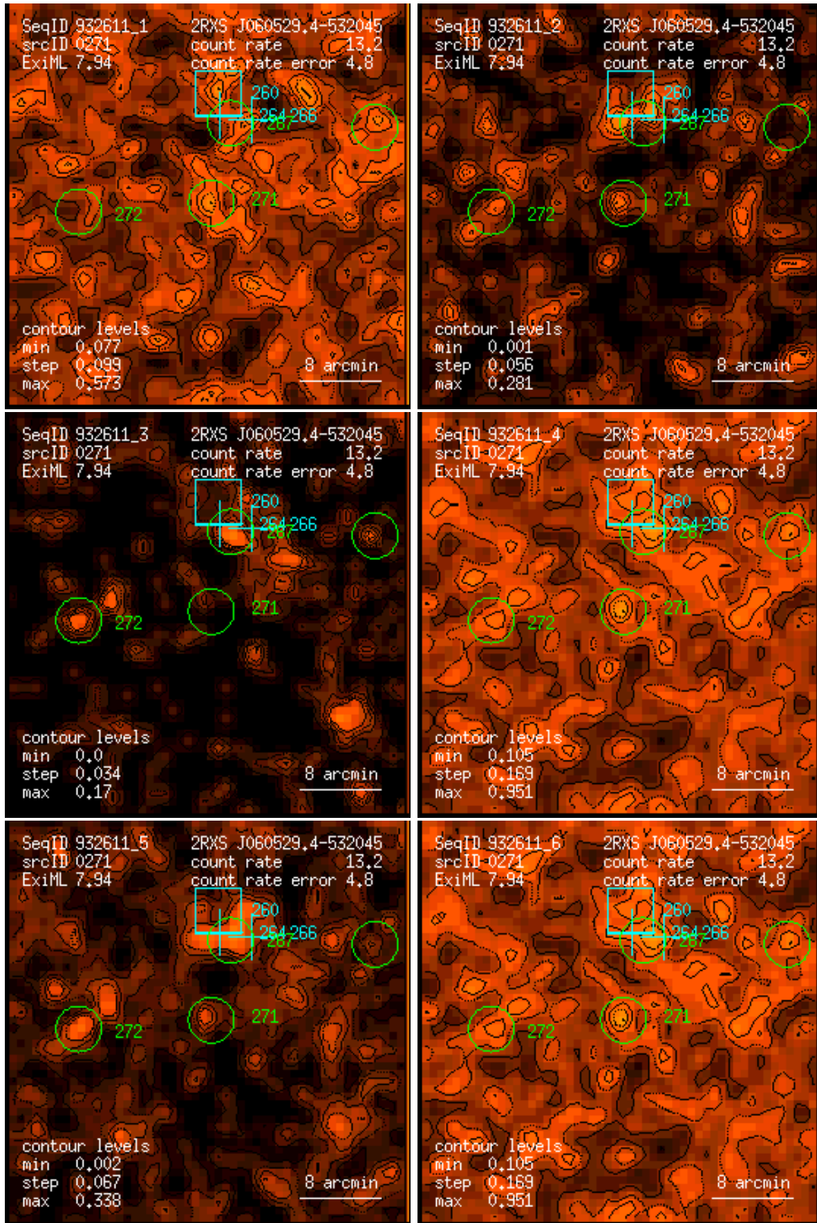
Figure 271: RASS 932611: detection 0271: band rate images, Gaussian filter: (1) PSPC channels 11 – 41, (2) 52 – 90, (3) 91 – 201, (4) 11 – 235, (5) 52 – 201, (6) 11 – 201. Broad band rates in counts/ks. Band rate contour levels in counts/ks/arcmin 2 .
