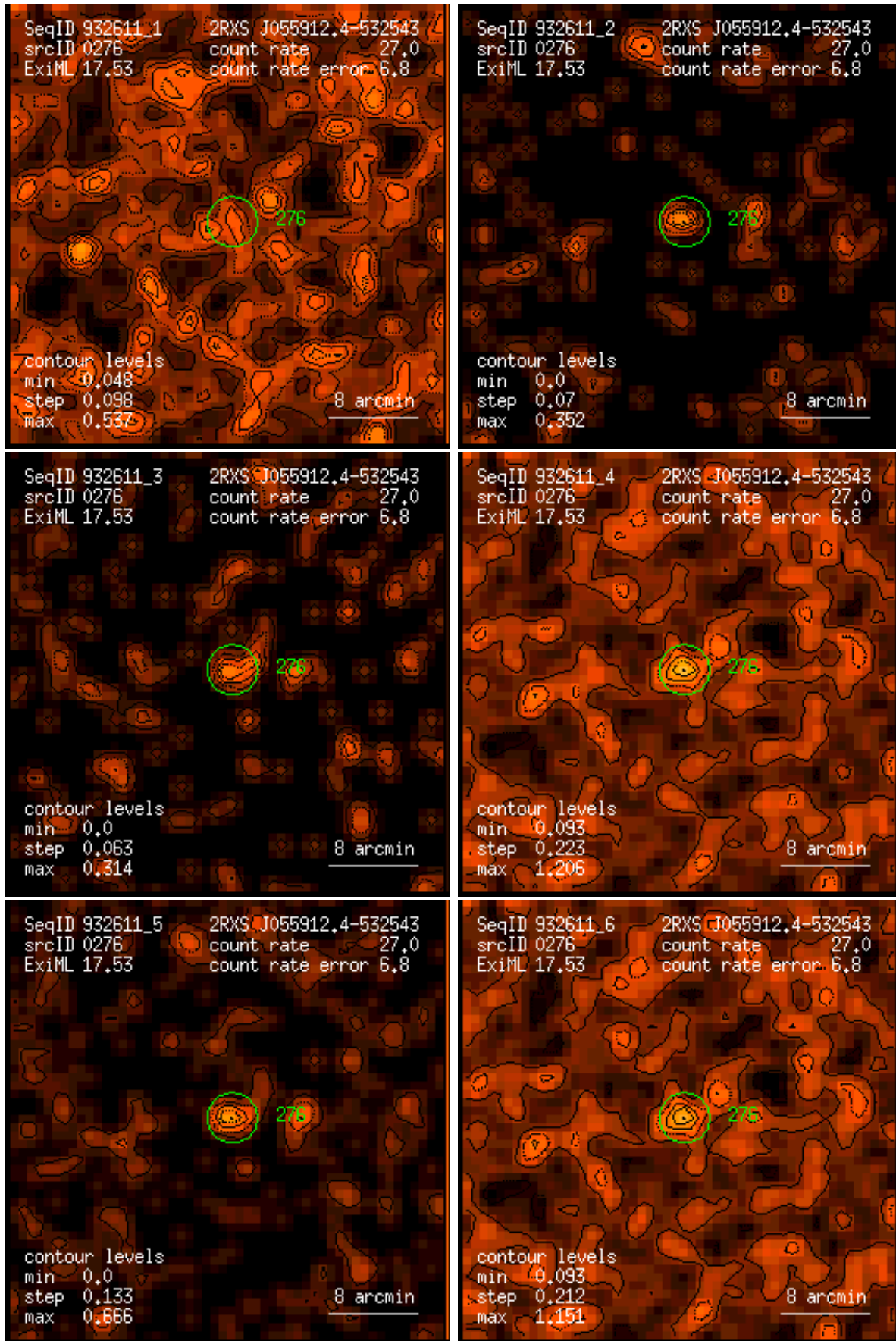
Figure 276: RASS 932611: detection 0276: band rate images, Gaussian filter: (1) PSPC channels 11 – 41, (2) 52 – 90, (3) 91 – 201, (4) 11 – 235, (5) 52 – 201, (6) 11 – 201. Broad band rates in counts/ks. Band rate contour levels in counts/ks/arcmin 2 .
