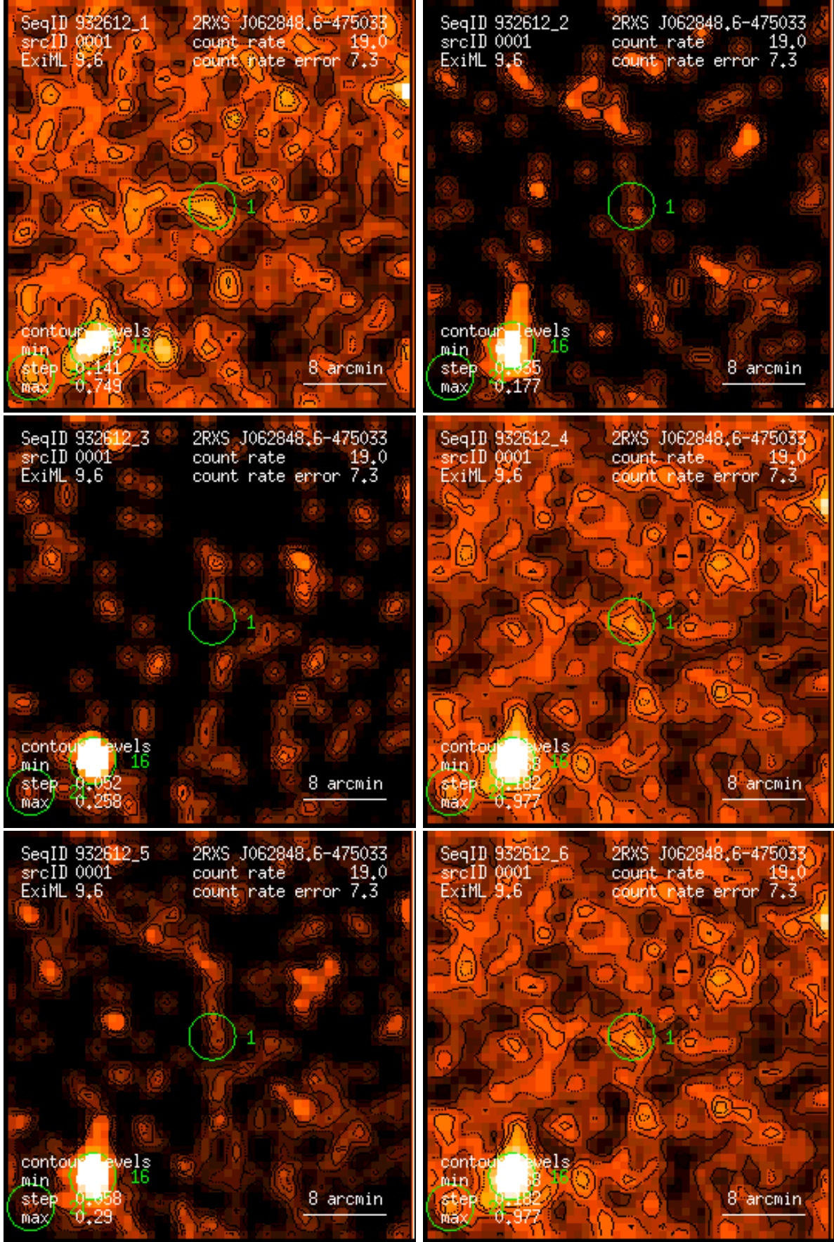
Figure 1: RASS 932612: detection 0001: band rate images, Gaussian filter: (1) PSPC channels 11 – 41, (2) 52 – 90, (3) 91 – 201, (4) 11 – 235, (5) 52 – 201, (6) 11 – 201. Broad band rates in counts/ks. Band rate contour levels in counts/ks/arcmin 2 .
