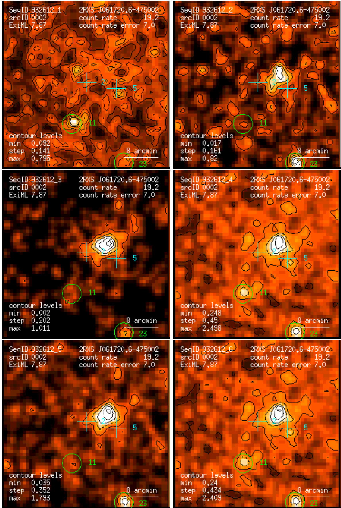
Figure 2: RASS 932612: detection 0002: band rate images, Gaussian filter: (1) PSPC channels 11 – 41, (2) 52 – 90, (3) 91 – 201, (4) 11 – 235, (5) 52 – 201, (6) 11 – 201. Broad band rates in counts/ks. Band rate contour levels in counts/ks/arcmin 2 .
