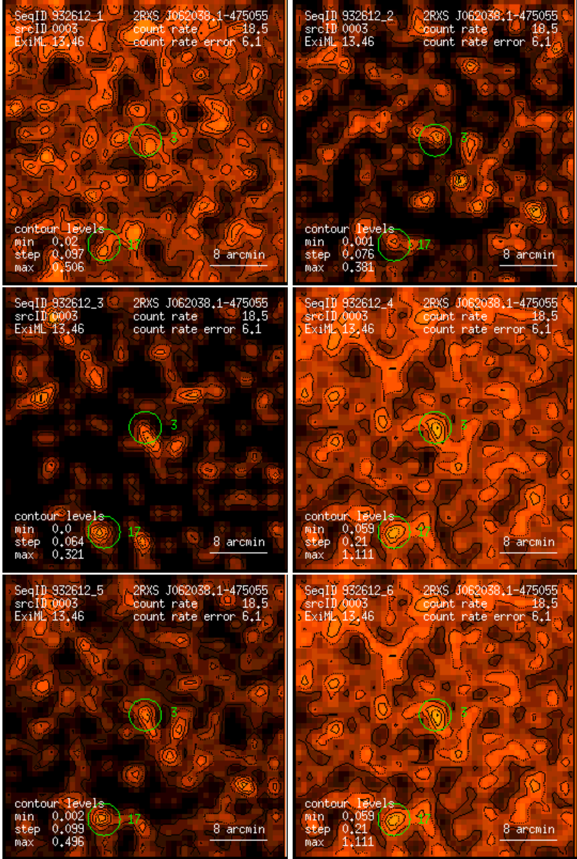
Figure 3: RASS 932612: detection 0003: band rate images, Gaussian filter: (1) PSPC channels 11 – 41, (2) 52 – 90, (3) 91 – 201, (4) 11 – 235, (5) 52 – 201, (6) 11 – 201. Broad band rates in counts/ks. Band rate contour levels in counts/ks/arcmin 2 .
