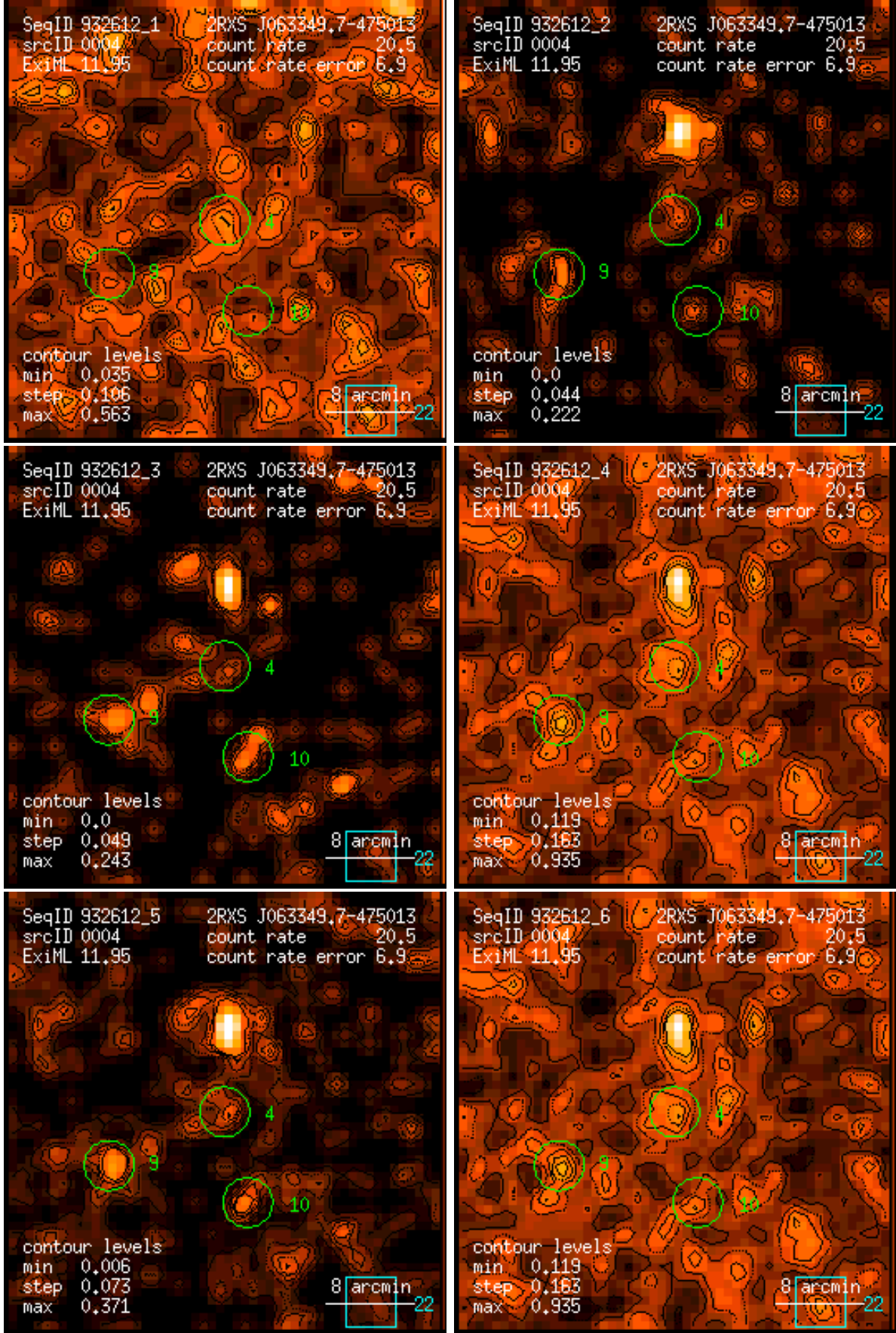
Figure 4: RASS 932612: detection 0004: band rate images, Gaussian filter: (1) PSPC channels 11 – 41, (2) 52 – 90, (3) 91 – 201, (4) 11 – 235, (5) 52 – 201, (6) 11 – 201. Broad band rates in counts/ks. Band rate contour levels in counts/ks/arcmin 2 .
